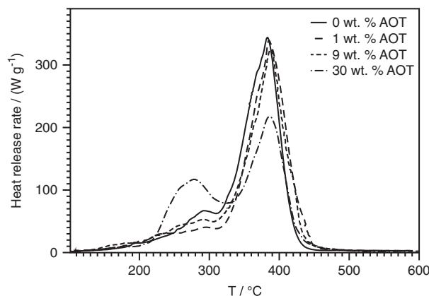
Figure 5 Representative plots of heat release rate versus temperature for each of the AOT-containing composites. A full colour version of this figure is available at the Polymer Journal journal online.
