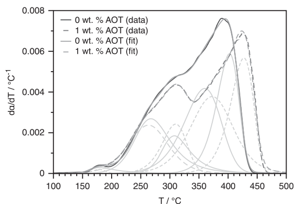
Figure 4 The derivative of the TGA data ( da/dT ) as a function of temperature for PMMA homopolymer and the 1 wt. % AOT composite fit to equation (4). The data for both can be fit using a five-step degradation. The first three steps are similar, but the final two steps at highest temperatures, plausibly corresponding to random chain scission, are shifted to higher temperatures for the AOT-containing composite. A full colour version of this figure is available at the Polymer Journal journal online.
