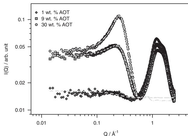
Figure 8 X-ray scattering data of AOT dispersed in MMA at several AOT concentrations. The data are well described by a spherical form factor 53,54 with a hard-sphere structure factor. 55,56 The radii of the spheres measured by X-ray scattering (the sodium-containing polar cores) are approximately 8 nm in diameter, and the thicknesses of the shells are 2–3 nm. A full colour version of this figure is available at the Polymer Journal journal online.
