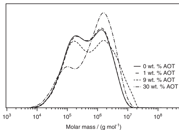
Figure 2 GPC chromatograms of PMMA-AOT composites in THF against PMMA standards. As the polymerization is not controlled, the molar mass distributions are broad. The pure PMMA and the 1 wt. % AOT sample are very similar; a small amount of surfactant does not impact the polymerization reaction. The 9 and 30 wt. % AOT samples are different; the distribution is shifted to larger species for both. GPC, gel permeation chromatography. A full colour version of this figure is available at the Polymer Journal journal online.
