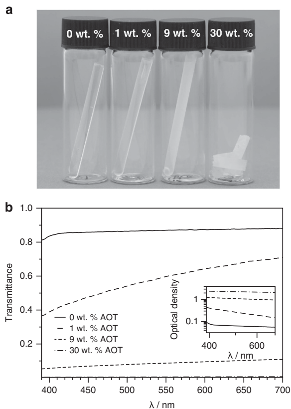
Figure 1 Optical properties of PMMA-AOT composites. (a) Optical image of PMMA-AOT composites (0, 1, 9, and 30 wt. % AOT, left to right). (b) Transmittance of visible light through PMMA-AOT composites as a function of wavelength ( \lambda from 390 to 700 nm). The curve for the sample containing 30 wt. % AOT is along the axis of the plot. The inset shows optical density as a function of wavelength \lambda , required for quantitative analysis of Tyndall scattering. 23–26 PMMA without any additive is highly transparent, and the addition of a small amount of AOT (1 wt. %) decreases the transparency slightly. Composites with higher concentrations of AOT are nearly opaque. A full colour version of this figure is available at the Polymer Journal journal online.
