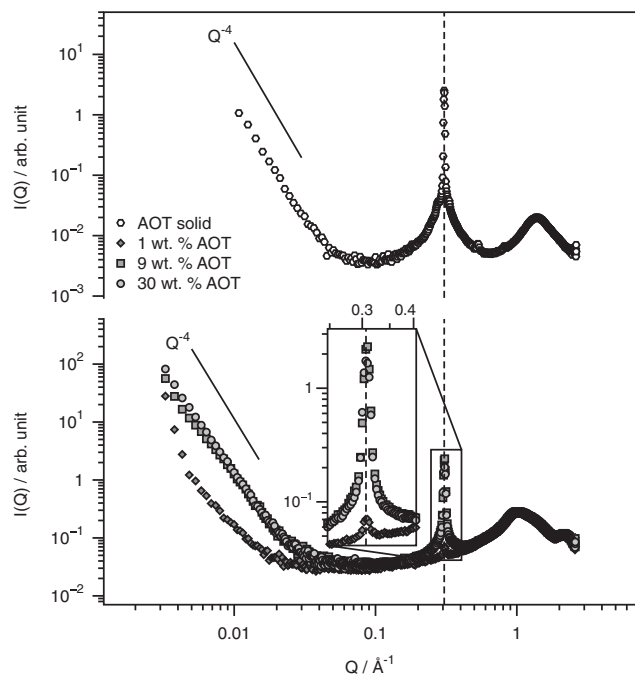
Figure 7 X-ray scattering data of anhydrous AOT solid (top) as well as PMMA-AOT composites at several AOT concentrations (bottom). Both sets of data consist of three regions: scattering proportional to Q^{-4} at low- Q due to long-ranged smooth interfaces, a peak at Q=0.3 \text{ \AA}^{-1} due to a reverse hexagonal phase, and peaks at high- Q due to short-ranged liquid-like order. The peak at Q=0.3 \text{ \AA}^{-1} in all the samples shows that the AOT phase separates into reverse hexagonal phase regions in the PMMA-AOT composites. The intensity of the scattering from the peaks in the PMMA-AOT composites shows that there is a lower concentration of self-assembled AOT in the 1 wt. % composite, as would be expected, but that there is the same amount of self-assembled AOT in the 9 and 30 wt. % composites. A full colour version of this figure is available at the Polymer Journal journal online.
