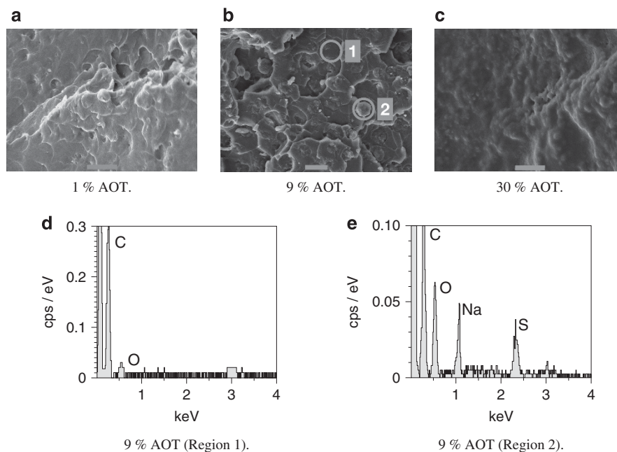
Figure 6 SEM micrographs (a–c) of PMMA-AOT composites with different concentrations of AOT and EDX spectra (d and e) of surfactant-free and surfactant-rich regions of the PMMA-AOT composite with 9 wt. % AOT. The regions that the EDX spectra were taken from are shown in (b). Scale bars in SEM micrographs denote 10 \mu\text{m} . A full colour version of this figure is available at the Polymer Journal journal online.
