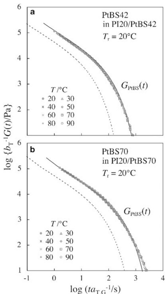
Figure 9 Test of time-temperature superposability for the G_{\text{PtBS}}^{\text{blt}}(t) data of (a) PtBS42 and (b) PtBS70 in the blends as indicated. The dotted curves show the G(t) of these poly( p-tert -butyl styrene) (PtBS) chains in the entanglement-free, iso- \tau_s reference state. For further details, see the text.
