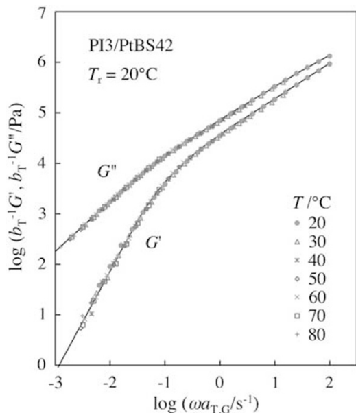
Figure 7 Viscoelastic behavior of PI3/PtBS42 blend ( w_{PI}=55.7 wt%) at T_r=20 °C.
