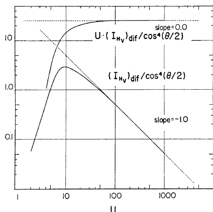
Figure 7. Plots of U \cdot (I_{H_V})_{\text{dif}} / \cos^4(\theta/2) and (I_{H_V})_{\text{dif}} / \cos^4(\theta/2) vs. U for the anisotropic one-dimensional rod in three-dimensional space. (I_{H_V})_{\text{dif}} = |I_{H_V}(\mu=0^\circ) - I_{H_V}(\mu=45^\circ)| , U = 4\pi(L/\lambda) \sin(\theta/2) and U^* = 50 .
