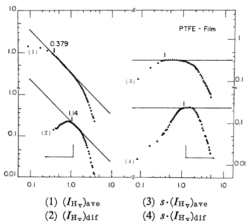
Figure 11. Measured intensity distributions (I_{H_V})_{ave} (curve 1), (I_{H_V})_{dif} (curve 2), s(I_{H_V})_{ave} (curve 3), and s(I_{H_V})_{dif} (curve 4) with s=(2\pi/\lambda)\sin\theta for poly(tetrafluoroethylene) film PTFE-L-ii.
