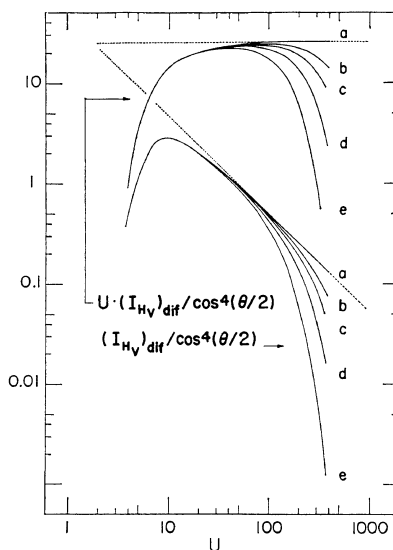
Figure 10. Plots of U(I_{H_V})_{\text{dif}} / \cos^4(\theta/2) and (I_{H_V})_{\text{dif}} / \cos^4(\theta/2) for the anisotropic rod in three-dimensional space. The radius of the rod R is set to be (a) R/L=0 , (b) 0.68 \times 10^{-2} , (c) 0.92 \times 10^{-2} , (d) 1.1 \times 10^{-2} , and (e) 1.7 \times 10^{-2} .
