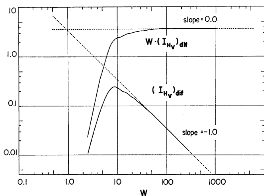
Figure 8. Plots of W \cdot (I_{H_V})_{\text{dif}} and (I_{H_V})_{\text{dif}} vs. W for the anisotropic one-dimensional rod in the two-dimensional space. W = 2\pi(L/\lambda) \sin \theta and W^* = 50 .
