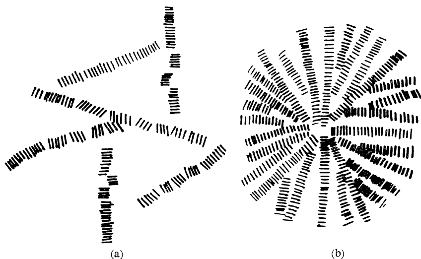
Figure 3. Schematic representations of orientation fluctuation and correlation of optical axes (indicated by lines) of anisotropic scattering elements; (a) rodlike orientation correlation, and (b) spherulitic orientation correlation.
