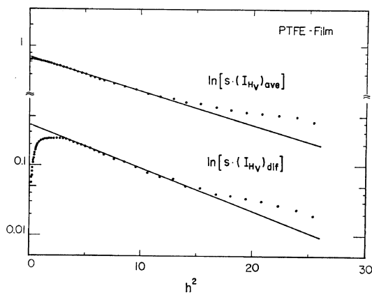
Figure 12. Guinier plots for the cross-sectional area of the rodlike particle for the PTFE-L-ii specimens; \ln[s(I_{H_V})_{ave}] , \ln[s(I_{H_V})_{dif}] vs. h^2 .
