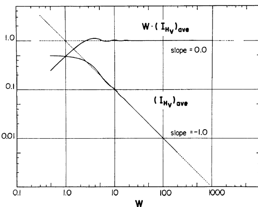
Figure 9. Plots of W(I_{H_V})_{\text{ave}} and (I_{H_V})_{\text{ave}} vs. W for the anisotropic one-dimensional rod in the two-dimensional space. (I_{H_V})_{\text{ave}} = |I_{H_V}(\mu=0^\circ) + I_{H_V}(\mu=45^\circ)|/2 , and W^* = 15 .
