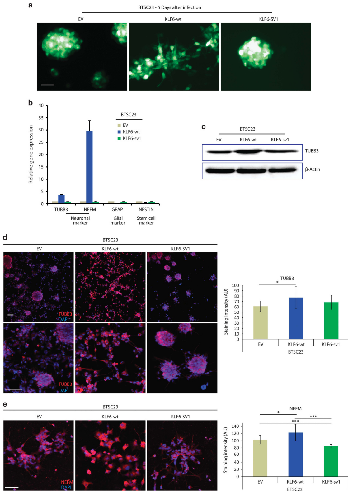
Figure 6. Wild-type KLF6 induces neural-like differentiation in BTSC23 cells. (a) Microphotographs of GFP-positive BTSC23 cells expressing empty vector (EV), KLF6-wt or KLF6-sv1, after lentiviral infection. (b) qRT-PCR analysis of neuronal ( TUBB3 , NEFM ), astrocytic ( GFAP ) and stem cell ( NESTIN ) markers in BTSC23 cells expressing EV, KLF6-wt or KLF6-sv1. (c) Immunoblotting of TUBB3 in BTSC23 cells expressing EV, KLF6-wt or KLF6-sv1. (d) Immunofluorescence staining and relative quantification for TUBB3 in BTSC23 cells expressing EV, KLF6-wt or KLF6-sv1. Nuclei were stained with DAPI. (e) Immunofluorescence staining using Tyramide Signal Amplification and relative quantification for NEFM in BTSC23 cells expressing EV, KLF6-wt or KLF6-sv1. Nuclei were stained with DAPI. * P < 0.05 , *** P < 0.001 . The scale bar represents 50 \mu\text{m} ( a , e ) or 100 \mu\text{m} ( d ). Relative gene expressions are normalized to EV, a representative qRT-PCR of three independent experiments is shown ( b ). Error bars represent mean \pm s.d.; n = 10 in d-e .
