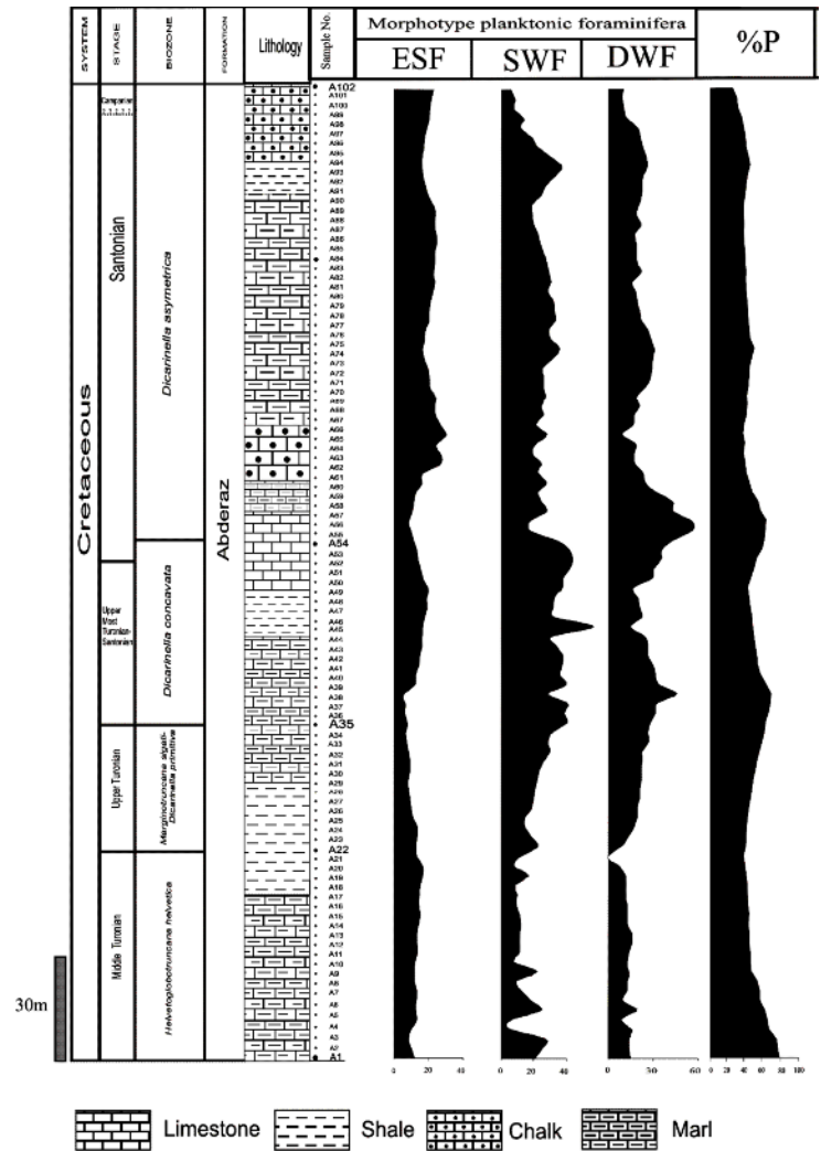
Fig2-Comparison of planktonic morphotype curves with %P ) ESF = Epicontinental Sea Forms, SWF = Shallow Water Forms, DWF = Deep Water Forms, %P =percentage of planktonic foraminifera)
