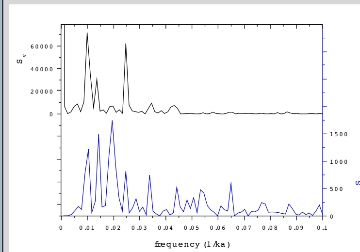
Figure 4. Power spectra for deuterium composition and its nonstationarity factor.
