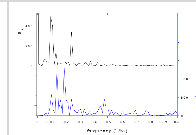
Figure 5. Power spectra for dust flux and its nonstationarity factor.
