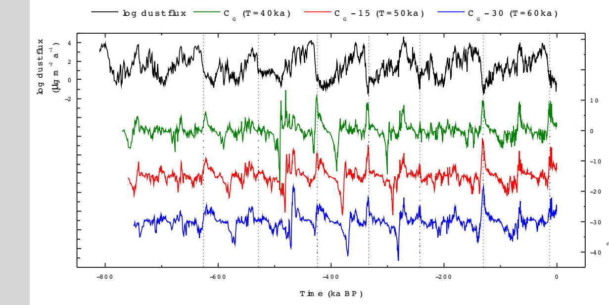
Figure 3. Dust flux and its FNS nonstationarity factors at three different averaging intervals.
