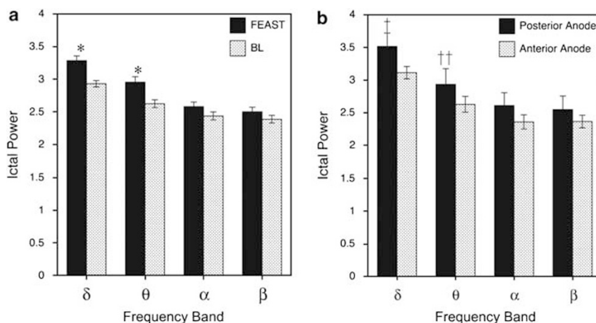
Figure 3 Ictal EEG power ( \log_{10}(\mu V^2) ) by condition and frequency band. (a) Combined data from Studies 1 and 2. FEAST had higher ictal power than BL in the slower frequency bands ( *p < 0.01 ). (b) In Study 2, polarity affected ictal power with unidirectional FEAST. Ictal power was higher in the slower frequency bands with the large posterior anode in comparison with the small anterior anode placement ( ^{\dagger}p < 0.003 , ^{\ddagger}p < 0.05 ).
