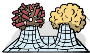
Majorana Permions
