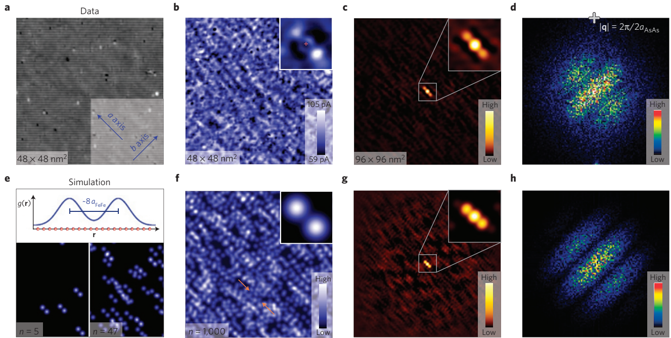
Figure 2 | Visualizing the anisotropic impurity state structure in Ca-122. a , A 48 nm × 48 nm topographic image of the Ca-122 surface, taken simultaneously with the measurements depicted in b–d . The horizontal lines stem from a surface reconstruction and do not influence our ability to visualize the correct FeAs electronic structure; the orientations of crystal axes are identified. b , The simultaneously recorded non-dispersive component in the electronic structure as determined the current map I(\mathbf{r}, E) at E = -37 meV. The inset shows the characteristic non-dispersive electronic structure environment of a typical Co-dopant atom (see Supplementary Sections SV and SVI): it is observed directly to be a ‘dimer’-shaped electronic impurity state. c , The autocorrelation of I(\mathbf{r}, -37 meV) shows three peaks separated by the characteristic length scale of 22 Å. Note that, apart from the triple-peak, the AC\{I(\mathbf{r}, -37 meV)\} signal is low, proving that 22 Å is the only persistent length scale in the image. d , Fourier transform I(\mathbf{q}, -37 meV) of the image shown in b . No sharp peaks indicating a periodic structure are seen anywhere in reciprocal space. e , Inset, the proposed impurity state with the Fe-lattice for comparison. The lower half show simulations with n = 5 and n = 47 . f , A simulation with n = 1,000 anisotropic impurity states in the same 48 nm × 48 nm FOV (Supplementary Section SIV); their centres are randomly distributed but they are all aligned with the a axis. This ‘glassy’ pattern of overlapping anisotropic impurity states looks similar to the data shown in b–d . The autocorrelation and Fourier transform ( g,h ) of the image in f support the validity of our deduction that the static electronic disorder consists of a axis oriented electronic anisotropic impurity states only.
