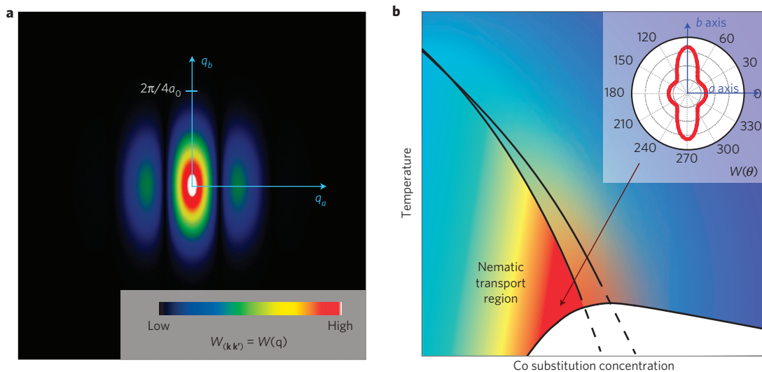
Figure 4 | Anisotropic transport due to scattering from anisotropic impurity states. a , False colour plot of the probability for a state \mathbf{k} to scatter into a state \mathbf{k}' , which in the Born approximation using plane waves is proportional to the Fourier transform of the scattering potential W(\mathbf{k},\mathbf{k}') = W(\mathbf{q}) \sim |FT\{V(\mathbf{r})\}|^2 . We take the scattering potential to have the same spatial form as the observed anisotropic impurity states (Fig. 2), with parameters for our model obtained from the experimental data. This then leads to the depicted C_2 -symmetric scattering probability W(\mathbf{q} = \mathbf{k} - \mathbf{k}') . b , A schematic phase diagram of 122 FeAs superconductors with increasingly nematic transport is indicated by blue, yellow and red colours, where the latter marks strongest transport anisotropy. To emphasize the directional dependence of the scattering probability from our QPI data, we plot in the inset the cumulative scattering probability in a given direction \theta = \angle(\mathbf{k},\mathbf{k}') . This is obtained by integrating over the radial coordinate: W(\theta) = \int d|\mathbf{q}| W(\theta, |\mathbf{q}|) in a . Note the strong scattering maxima along the b axis.
