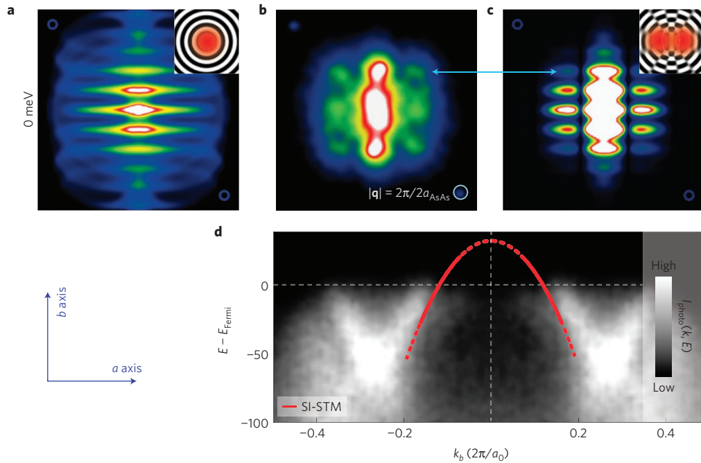
Figure 3 | Anisotropic QPI from anisotropic impurity states. (See Supplementary Section SVII for a comparison of \mathbf{q} - and \mathbf{k} -space.) a , The QPI pattern one would expect from the ARPES band structure (Fig. 1e and Supplementary Section SII) with the quasiparticles scattering from point-like scatterers. b , The QPI pattern as measured in Ca-122 in the same energy range. Although the dispersion is correct, there are clear vertical lines of suppressed intensity in the data, which are not visible in the simulations. c , Using the structure factor of a ‘dimer’ (Fig. 2) impurity state, the calculations yield QPI predictions consistent with the data in b (see for example blue line). d , The dispersion of the measured QPI (red line) is in agreement with the dispersion determined by ARPES (photocurrent intensity in grey scale).
