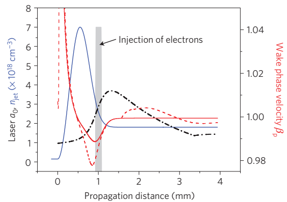
Figure 3 | Simulated evolution of the normalized vector potential a_0 (dash-dot line) as a function of propagation distance for \Delta x_f = 1.6 mm and n_{\text{jet}} = 7 \times 10^{18} \text{ cm}^{-3} . The blue solid line shows the longitudinal density profile. The phase-velocity reduction (red dashed line) was larger than that for the down-ramp alone (red solid line) owing to self-focusing increasing the nonlinear plasma wavelength, and trapping of electrons occurred in the grey shaded area. The phase velocities shown are measured in the centre of the bubble behind the laser pulse, where the longitudinal electric field is zero. The phase-velocity reduction at the back of the bubble is approximately a factor of two larger.
