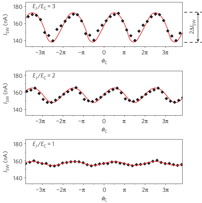
Figure 3 | Measured switching current (black diamonds) as a function of \phi_C over the chain for three different E_J/E_C ratios. The measurement noise for each point is about 0.2 nA. The red lines represent theoretical calculations for the switching current using equations (3) and (2).
