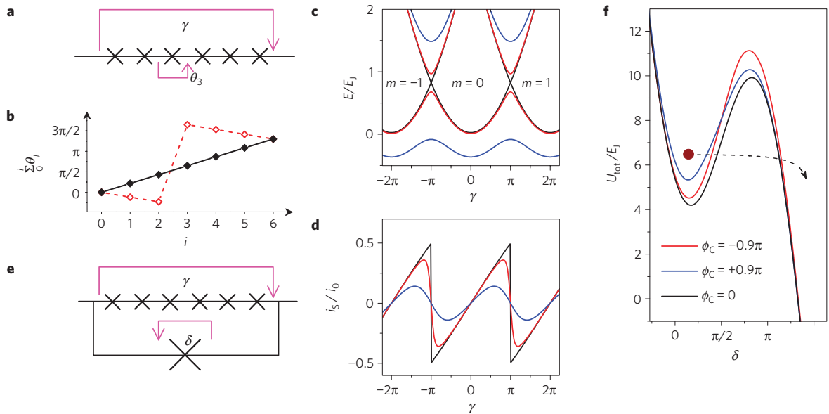
Figure 1 | Graphic representations describing the effect of phase slips in a six-junction chain, the resulting chain's energy and supercurrent and the measurement principle. a , Schematic picture of the phase-biased Josephson junction chain. b , Representation of a phase slip in the chain. The filled diamonds show the initial configuration. The open diamonds show the phase configuration after a 2\pi flip of the phase on the third junction \theta_3 . c , Energy levels of a Josephson junction chain with N = 6 as a function of bias phase \gamma for different ratios E_J/E_C . For E_J/E_C = 20 (black lines) no splitting is visible at the crossing points. For E_J/E_C = 3 (red lines) a gap emerges that increases rapidly with decreasing E_J/E_C . The blue lines show the energy levels for E_J/E_C = 1.3 . For each E_J/E_C , the two lowest-lying states have been calculated by numerical diagonalization of the Hamiltonian (1). d , Current-phase relation for the ground state E_g(\gamma) for the same E_J/E_C ratios as in c . The supercurrent is calculated from the derivative of the energy band: i_s = (2e/\hbar)(\partial E_g/\partial \gamma) . The chain current is reported in units of the critical current of a single chain junction i_0 = (2e/\hbar)E_J . e , Schematic picture of the chain shunted by the read-out junction. f , Escape potential for the Josephson junction chain with E_J/E_C = 3 in parallel with the read-out junction for three different flux biases \phi_C in the read-out loop (see Fig. 2). The ground state of the chain clearly modifies the escape potential of the read-out junction.
