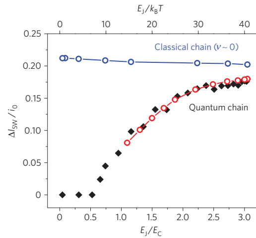
Figure 4 | Comparison between the measured and the calculated switching-current amplitude as a function of the E_J/E_C ratio. Black diamonds: measured; red open circles: calculated. Note that the switching-current amplitude is divided by the flux-dependent critical current of a single SQUID i_0 , to reveal the effect of quantum-phase fluctuations. The top curve (blue open circles) shows the theoretical calculation of the switching-current amplitude in the absence of quantum phase fluctuations. The lines are guides for the eye.
