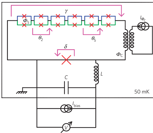
Figure 2 | Measurement circuit. The six-SQUID chain is inserted in a superconducting loop. The flux \Phi_C created by on-chip coils controls the phase difference \gamma over the chain. The flux \Phi_S through the SQUIDs can be controlled independently by a second coil. We denote the phase difference over the read-out junction \delta .
