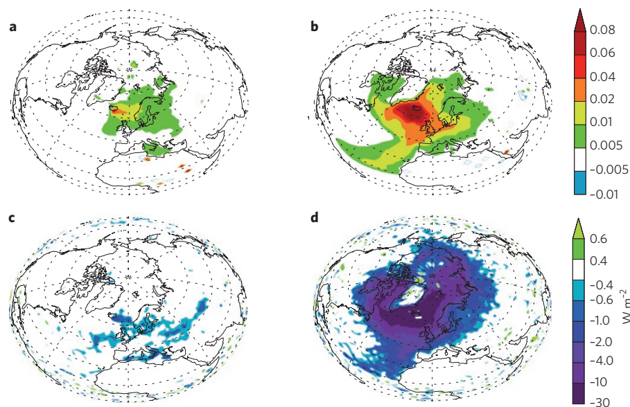
Figure 1 | Simulated changes due to the Nornahraun eruption in Iceland. a,b , Differences in aerosol optical depth ( \Delta\text{AOD} , unitless) at visible wavelengths (550 nm) between simulations with and without volcanic sulfur dioxide emissions during September–November ( a ) and June–August ( b ). c,d , Differences in radiative flux at the top of the atmosphere ( \Delta\text{TOA} ) for the same simulations, for September–November ( c ) and June–August ( d ).
