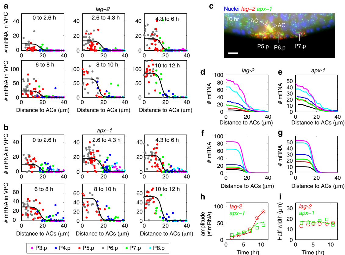
Figure 4 | Graded Notch ligand expression dynamics in lin-12/Notch mutant animals. (a) Level of lag-2 mRNA in all VPCs as function of the distance of each VPC to the ACs for different stages of induction as characterized by gonad length ( n = 111 animals). Markers indicate expression levels in P3.p (magenta), P4.p (blue), P5.p (red), P6.p (grey), P7.p (green) and P8.p (cyan). Lines indicate best fit of equation (3) to the data. (b) Same as in (a) but for apx-1 . (c) Visualization of individual lag-2 (red) and apx-1 (green) mRNA molecules in a lin-12(lf) mutant, showing high Notch ligand expression in P5.p, P6.p and P7.p during late vulva induction. Scale bar, 5 \mu\text{m} . (d,e) Sliding averages of the expression level of lag-2 (d) and apx-1 (e) for 0–2.6 h (black), 2.6–4.3 h (red), 4.3–6 h (green), 6–8 h (blue), 8–10 h (cyan) and 10–12 h (magenta). Sliding averages were calculated with window size of 5 \mu\text{m} . (f,g) Best fit of the model in equation (3) to the different time points in panels a and b. (h) Amplitude as a function of time of the lag-2 (red) and apx-1 (green) spatial expression profile for the experimental data in panels (a) and (b) (markers) and the fit to equation (3) (dots). For the experimental data, the amplitude is calculated by an average over the expression levels in all VPCs within a distance < 5 \mu\text{m} of the AC. (i) Half-width of the lag-2 (red) and apx-1 (green) expression profile for the data in (a,b) (markers) and the fit to equation (3) (dots). The experimentally observed half-width is calculated from the sliding average in (d,e).
