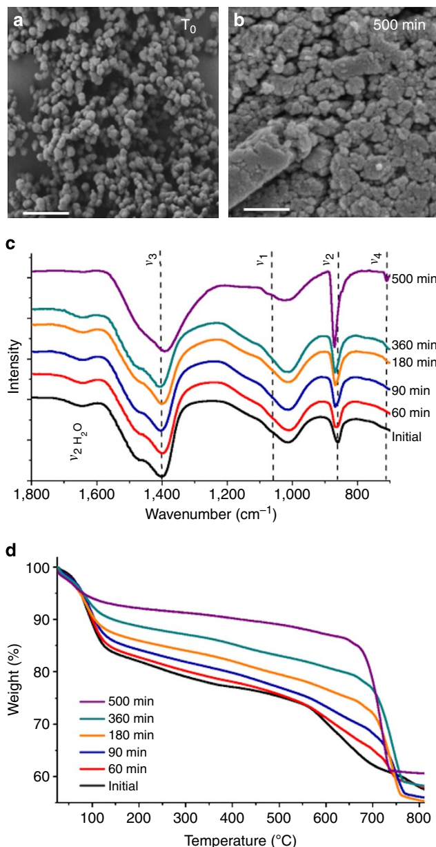
Figure 2 | Dehydration of ACC- \text{SiO}_2 particles on incubation in solution. SEM images of ACC- \text{SiO}_2 particles after incubation in solution for (a) 0 min and (b) 500 min—scale bar, 500 nm. (c) Infrared spectra and (d) thermogravimetric analyses of ACC- \text{SiO}_2 particles, showing the structural and compositional changes in the particles with incubation in solution.
