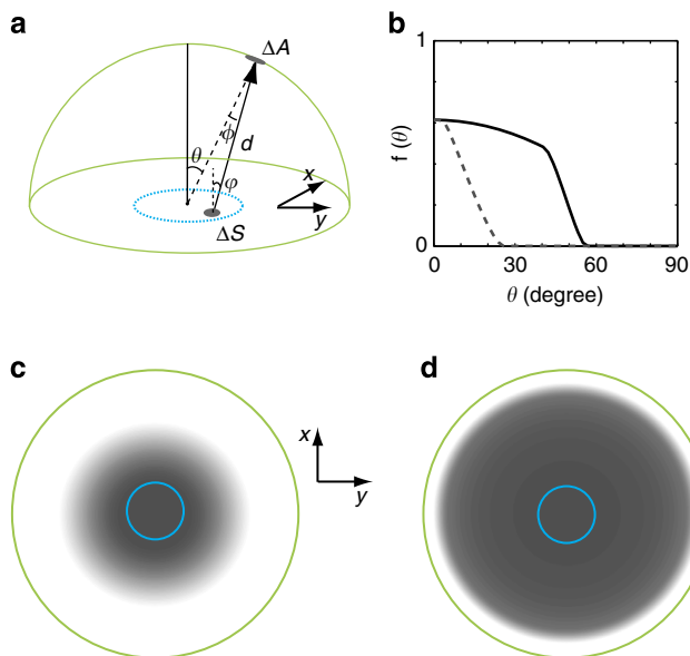
Figure 3 | Distribution of thermal radiation on the surface of the extraction dome. (a) Schematic of the calculation. Solid arrow indicates radiation that is emitted from a small area \Delta S on the cavity opening and is received by a small area \Delta A on the surface of the dome. (b) Distribution of the radiation power on the surface of the dome as a function of the polar angle \theta . Dashed and solid lines are for the cases with empty and filled cavities, respectively. (c,d) The distribution of the radiation power, plotted on the hemisphere of the dome, for the case of empty (c) and filled (d) cavity. The blue circle indicates the emitter area, that is, the opening area of the cavity. The green circle is the boundary of the dome. Darker region indicates higher emission and the white region has zero emission.
