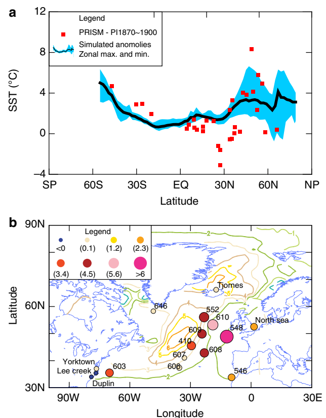
Figure 4 | Comparison between PRISM and simulated Atlantic SST.
