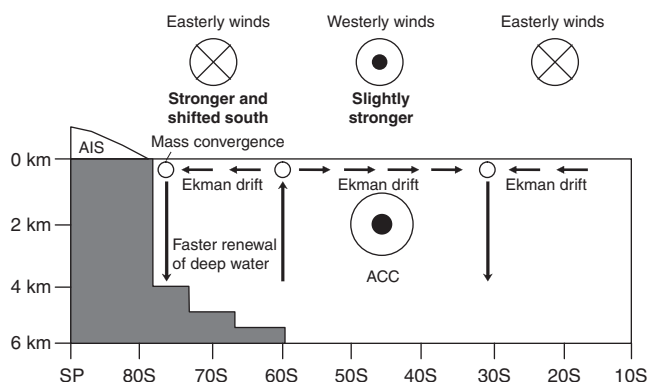
Figure 3 | Southern Ocean/South Atlantic dynamics during the mPWP.
