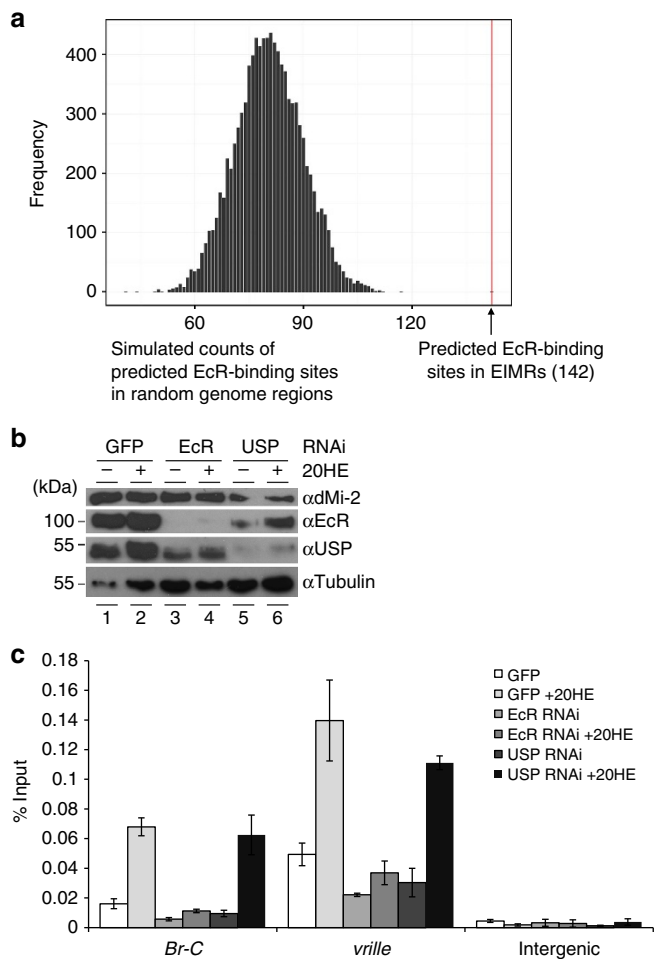
Figure 3 | EcR but not USP is essential for recruitment of dMi-2 to ecdysone-activated genes. (a) Enrichment of predicted EcR-USH binding sites in EIMRs. The histogram shows the distribution (sampled from 10,000 runs) of putative EcR-USH site number within the same number of randomly selected genomic regions with the same sizes as the experimentally determined EIMRs. The red line indicates the number of computationally identified EcR-USH binding motifs within EIMRs (142; P < 10^{-8} ). The P -value for the observed number of binding motifs was estimated from the normal distribution that can be approximated based on the displayed simulated distribution, that is, using mean and s.d. estimates from the simulated sample. (b) Western blot analysis of protein extracts of S2 cells treated with dsRNA directed against GFP (control), EcR or USP. Cells were either left untreated (–20HE) or were treated with ecdysone (+20HE). Antibodies used are shown on the right, molecular masses on the left. Tubulin served as a loading control. (c) dMi-2 binding to Br-C and vrille following EcR and USP depletion analysed by ChIP-qPCR. Chromatin was prepared from S2 cells that were first treated with dsRNA against GFP (control), EcR or USP and then either left untreated or were exposed to 1 \mu\text{M} ecdysone for 6 h as indicated. ChIP-qPCR was performed with dMi-2 antibody. Error bars denote s.d. of technical triplicates. Experiments were performed as biological triplicates. One representative example is shown.
