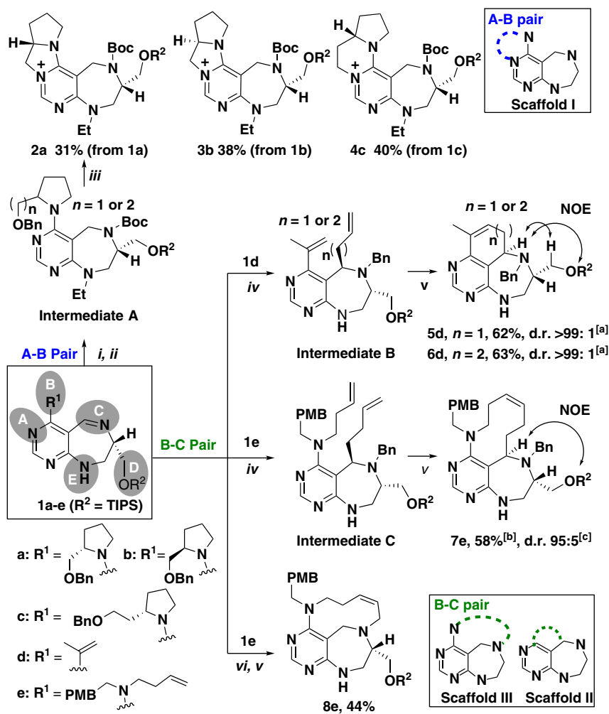
Figure 2 | A–B and B–C pairing pathways for synthesis of scaffolds I–III. Reagents and conditions: (i) \text{NaBH}_4 , MeOH, 0 °C → r.t. then \text{Boc}_2\text{O} , TEA, DCM, 0 °C → r.t.; (ii) EtI, NaH, DMF, 0 °C → r.t.; (iii) \text{Pd}(\text{OH})_2/\text{C} , \text{H}_2 , MeOH, then \text{MsCl} , TEA, DCM, 0 °C → r.t.; (iv) \text{BnBr} , ACN, 80 °C, then \text{RMgBr} , THF, –78 °C → r.t.; (v) Grubbs' second-generation catalyst (20 mol%), toluene, reflux; and (vi) \text{NaBH}_4 , MeOH, 0 °C → r.t., then allyl bromide, TEA, DMF, 0 °C → r.t. TIPS, triisopropylsilyl; TEA, triethylamine; \text{MsCl} , methanesulfonyl chloride; \text{BnBr} , benzyl bromide; ACN, acetonitrile. [a] Determined by LC–MS analysis of crude reaction mixture and by 1 H NMR analysis of samples purified by short silica-gel column. [b] Yield of the isolated major diastereomer. [c] Determined by LC–MS analysis of crude reaction mixture. 1 H NMR, proton nuclear magnetic resonance. LC–MS, liquid chromatography–mass spectrometry.
