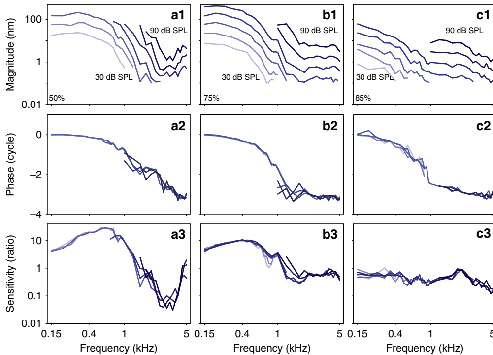
Figure 2 | Representative vibratory responses of the SHC/BM region. (a) 50% from the base. (b) 75% from the base. (c) 85% from the base. (Top) The vibratory magnitude. Magnitude responses at high sound levels and at low frequencies were not shown due to saturation of our system (explained in Methods). (Middle) The phase normalized to columella phase. (Bottom) The sensitivity was the magnitude of BM vibration divided by the vibratory magnitude of the columella.
