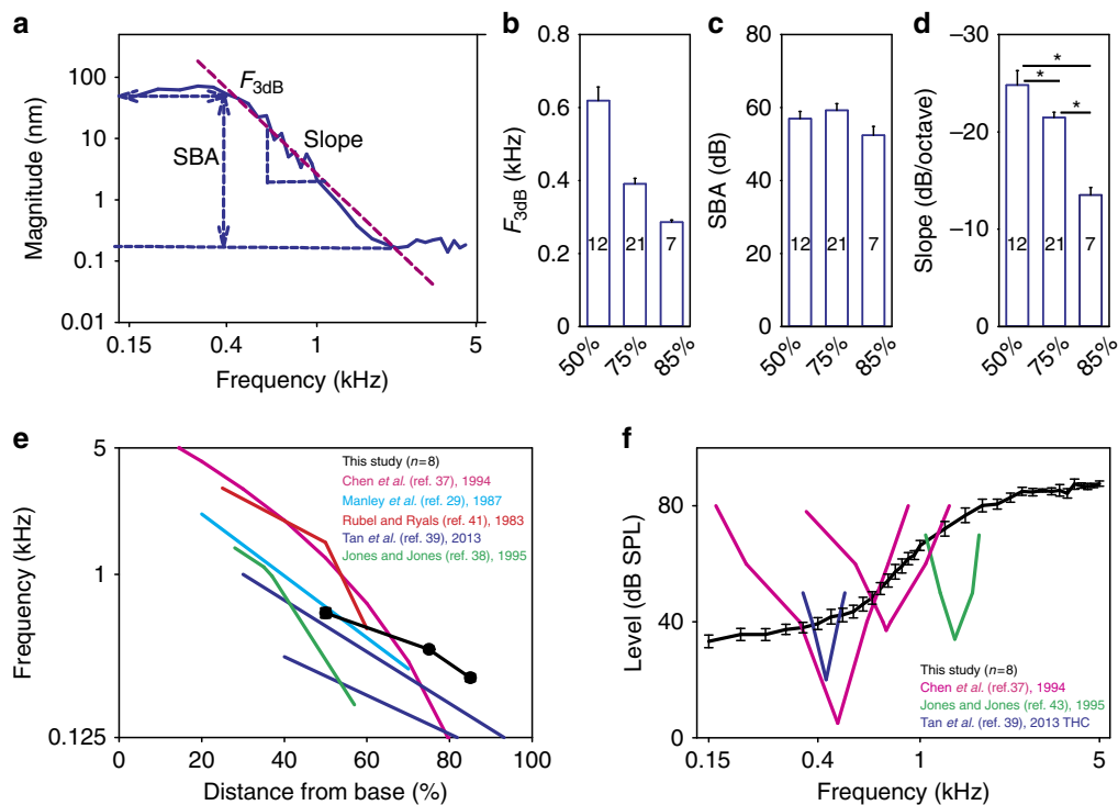
Figure 3 | Mechanical responses do not match hair cell and auditory nerve responses. (a) The vibratory responses were fit with a low-pass filter model to calculate the corner frequency ( F_{3dB} , b ), the stop-band attenuation (SBA, c ), and the filter slope (slope, d ). (e) The tonotopic map we estimate using the corner frequencies was similar to previously published maps of the chicken basilar papilla. (f) The sound level needed to produce a 30 nm magnitude vibration at the 75% location was not tuned, unlike the threshold plots from previously published measurements in auditory nerve fibres and hair cells. Error bars show the s.e.m. Asterisks in d represent statistical significance *P < 0.05 .
