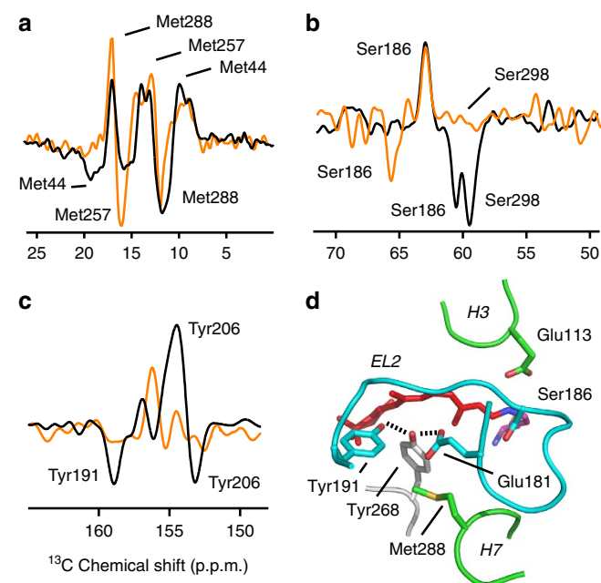
Figure 3 | Changes in EL2 interactions in Meta-I and Meta-II. 1D NMR difference spectra are shown of rhodopsin minus Meta-I (orange) and rhodopsin minus Meta-II (black) using rhodopsin containing labelled 13 Cε-Met (a), 13 Cβ-Ser (b) or 13 Cζ-Tyr (c). The rhodopsin spectra correspond to positive peaks, while the Meta-I and Meta-II spectra correspond to negative peaks. The assignments of the resonances have previously been reported 18,19,38,64 . (d) Crystal structure of rhodopsin in the region of Tyr268 6.51 (PDB-ID 1U19; ref. 26).
