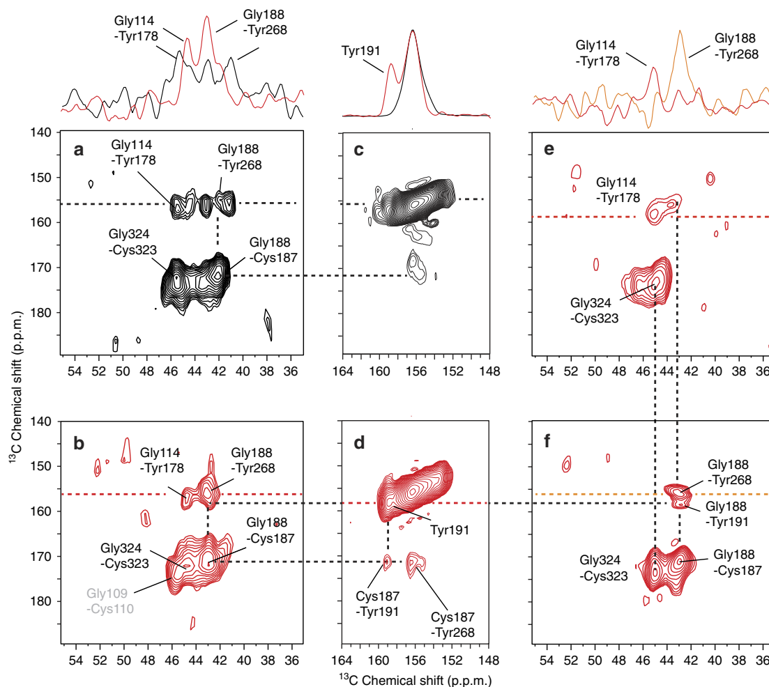
Figure 2 | Tyr268 6.51 to Gly188 EL2 and Tyr268 6.51 to Cys187 EL2 contacts in Meta-II. (a) 2D DARR spectrum highlighting Tyr-Gly contacts in rhodopsin using rhodopsin containing ^{13}\text{C} -Tyr, ^{13}\text{C} -Gly and ^{13}\text{C} -O-Cys. In the rhodopsin crystal structure (PDB-ID 1U19; ref. 26), there are six Tyr(C \zeta )-Gly(C \alpha ) contacts, which are all located in the extracellular region of rhodopsin. These contacts involve five tyrosines and five glycines: Tyr10 N-term -Gly3 N-term , 3.9 Å; Tyr10 N-term -Gly280 EL3 , 4.4 Å; Tyr29 N-term -Gly101 EL1 , 4.0 Å; Tyr178 EL2 -Gly114 3.29 , 4.5 Å; and Tyr191 EL2 -Gly188 EL2 , 5.2 Å; and Tyr268 6.51 -Gly188 EL2 , 5.3 Å. Above a are shown rows through the Tyr-Gly crosspeaks. The rows better illustrate the intensity change occurring in the Tyr268 6.51 -Gly188 EL2 peak on activation. The observation that the Tyr178 EL2 -Gly114 3.29 crosspeak does not change intensity is consistent with the lack of influence of the Y178F mutation on the Meta-I-Meta-II transition (Fig. 4g). (b) Wild-type Meta-II spectrum using rhodopsin containing ^{13}\text{C} -Tyr, ^{13}\text{C} -Gly and ^{13}\text{C} -O-Cys. (c,d) Region of the 2D DARR spectra of rhodopsin (black) and Meta-II (red) corresponding to ^{13}\text{C} -Tyr to ^{13}\text{C} -O-Cys crosspeaks. Above c are shown rows through the ^{13}\text{C} -Tyr diagonal of rhodopsin and Meta-II. (e,f) G188A Meta-II and Y178F Meta-II spectra, respectively, using the same ^{13}\text{C} -labelling scheme as above. Rows are shown through the Tyr-Gly crosspeaks in the G188A Meta-II and Y178F Meta-II spectra above e .
