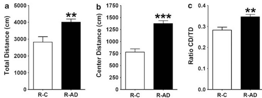
Figure 4 Interactions of recurrent restraint stress (RRS), short-term antidepressant treatment and fat diet on locomotor activity and anxiety. Open field tests were conducted after the period of RRS ended, each session lasted 60 min from days 14 to 67. (a) RRS-antidepressant treated group (R-AD) had increased total distance (TD) when compared with untreated RRS animals (R-C). (b) R-AD group had increased center distance (CD) when compared with R-C. (c) Anxiety was estimated by the ratio of center distance (CD) over TD; R-AD animals were significantly less anxious than R-C. Columns and bars (a–c) depict mean and s.e., respectively; ** P < 0.01 ; *** P < 0.0001 .
