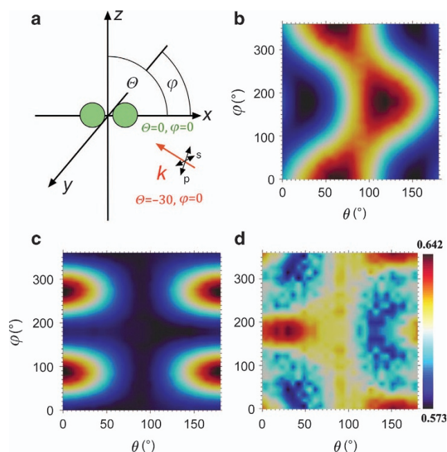
Figure 3 Dependence of the spectral response on the NP dimer orientation. (a) Geometric details of the simulations. The dimer comprises a pair of gold monomers, each of which had a diameter of 60 nm and was separated from each other by 10 nm. The long axis of the dimer was aligned with the x axis, and the light was incident with an oblique angle of \theta = -30^\circ ; \theta and \varphi are the polar and azimuthal angles in the text. (b) Calculated extinction cross-section at 530 nm for p-polarized light. (c) Calculated extinction cross-section at 530 nm for s-polarized light. (d) Normalized difference in polarization-averaged cross-section \Delta\sigma_{\text{norm}} between \lambda = 530 and 585 nm as a function of \theta and \varphi . NP, nanoparticle.
