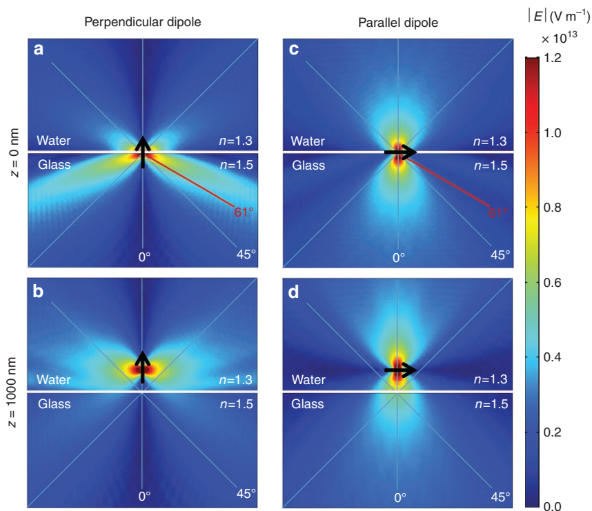
Figure 2 Angular distributions of the radiation emitted by a punctual incoherent dipole located at a distance ‘ z ’ from a water/glass interface ( \theta_c=61.1^\circ ). (a) Dipole oriented perpendicular to the interface at z=0 . In this case, a large amount of the radiated power is emitted at high angles towards the lower half-space (glass). (b) For z=1000 nm ( z>\lambda=632 nm), almost all of the emission occurs towards the upper half-space (water), because of total internal reflection. (c) Dipole oriented parallel to the interface at z=0 and (d) at z=1000 nm. Radiation patterns from ensembles of randomly oriented dipoles were computed by adding the patterns of parallel and perpendicular dipoles 29,30 .
