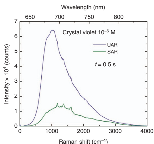
Figure 6 SAR detection of SERS. Because of the resonant excitation of crystal violet at 633 nm, both fluorescence emission and enhanced Raman scattering are produced and collected. The Raman signal from the coverslip surface is evident in the SAR spectrum, whereas the UAR spectrum is dominated by the fluorescence emission from the bulk solution.
