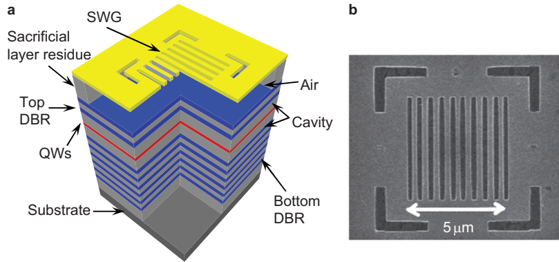
Figure 1 Examples of the hybrid cavity. (a) A schematic of a 0D hybrid cavity with a SWG mirror. (b) Top-view SEM image of a fabricated 0D cavity with a SWG of 5\ \mu\text{m} \times 5\ \mu\text{m} in size. 0D, zero-dimensional; SEM, scanning electron microscopy; SWG, subwavelength grating.
