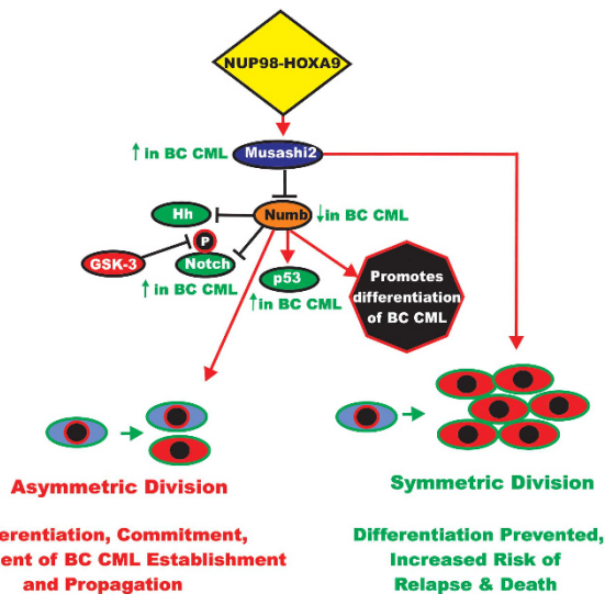
Figure 6. Roles of Musashi and Numb in regulation of asymmetric and symmetric cell division in BC CML. Chimeric upstream transcription factors such as NUP98-HOXA9 can induce the Musashi RNA binding factor that is important in determining cell fate. Musashi is elevated in BC CML; in contrast, the Numb protein is detected at low levels in BC CML. The Numb protein plays a key role in asymmetric cell division and it is usually present in one daughter cell after division and not the other, allowing different cellular fates. Numb can regulate many pathways important in BC CML including Hh, Notch and p53 that can also be regulated by GSK-3. This figure is presented to provide the reader an idea of the importance of regulation of asymmetric vs symmetric division in BC CML and how division can be regulated by Numb and upstream Musashi and NUP98-HOXA9 .
