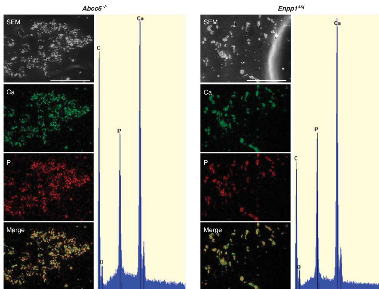
Figure 3 Energy dispersive X-ray analysis of the mineral deposits in the kidney of Abcc6 -/- and asj mice. The results revealed the presence of calcium and phosphorus as the principal ions in ~2:1 ratio. Topographic RADAR mapping of calcium (Ca) and phosphorus (P) revealed colocalization in merged images (scale bar, 1 mm).
