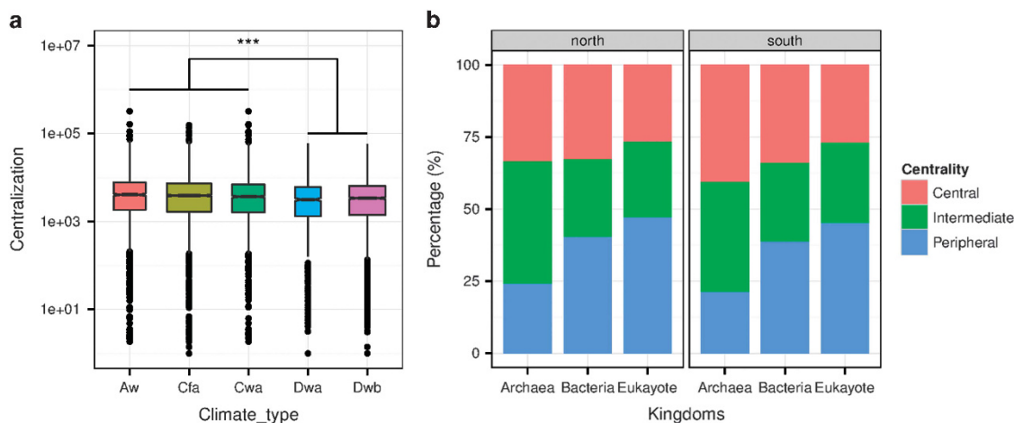
Figure 2 Betweenness centralization associated with different climatic regions (a) and percentage of bacterial, archaeal and fungal nodes with different centralization (b). *** P < 0.001 .
