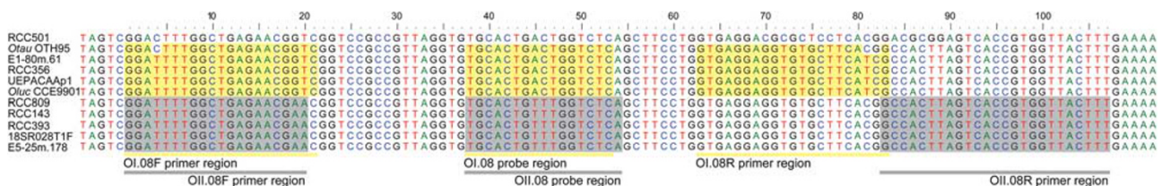
Figure 1 Regions of the 18S rRNA gene targeted by the Ostreococcus qPCR primer-probe sets. Three sequences (highlighted in grey) are from Ostreococcus Clade OII that were characterized as deep-adapted in Rodriguez et al. (2005), as well as two environmental clones. Five sequences are shown for Clade OI (highlighted in yellow), composed of O. tauri and the four other sequences, two from cultures and two from environmental samples (including sequences from two of the clades identified in Rodriguez et al., 2005 as being more high-light adapted). RCC501 represents the third putatively high-light adapted clade and is not targeted by either primer-probe set. Where highlighted sequences have perfect identity to respective primers and probes.
