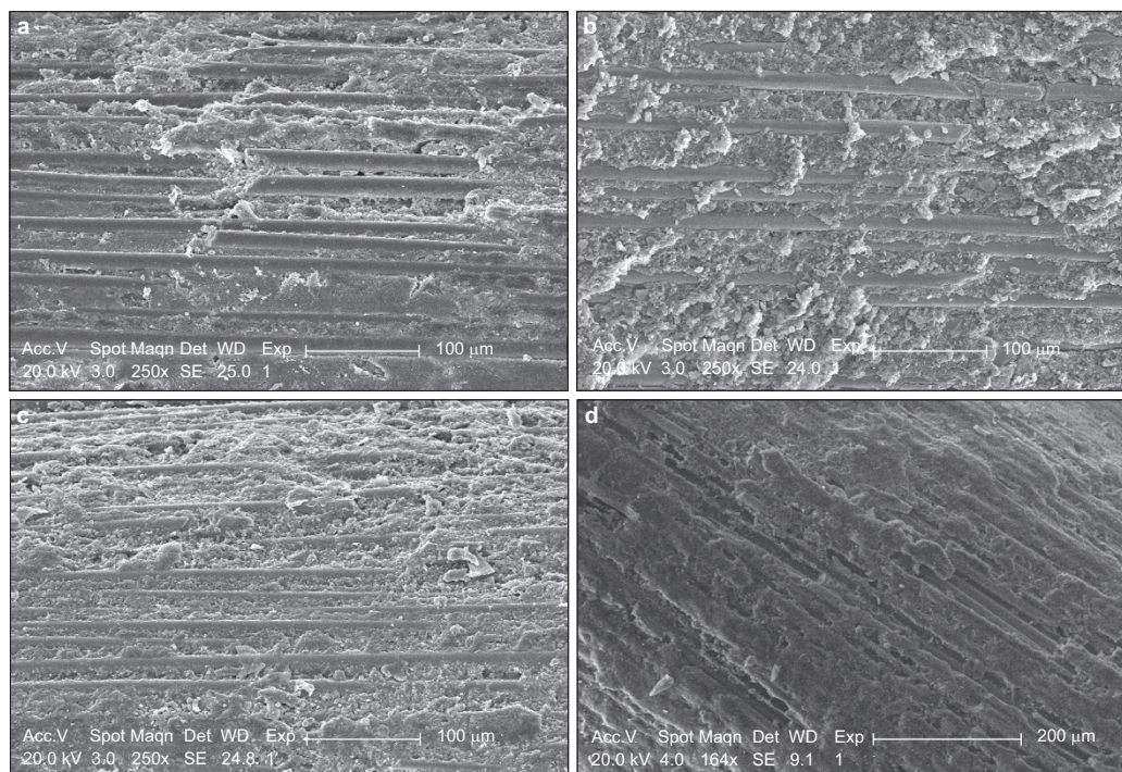
Figure 1 Microstructure of glass fiber post. (a) Without pre-treatment; (b) with pre-treatment of sandblasting; (c) with pre-treatment of sandblasting followed by silanization; (d) with pre-treatment of silanization.
