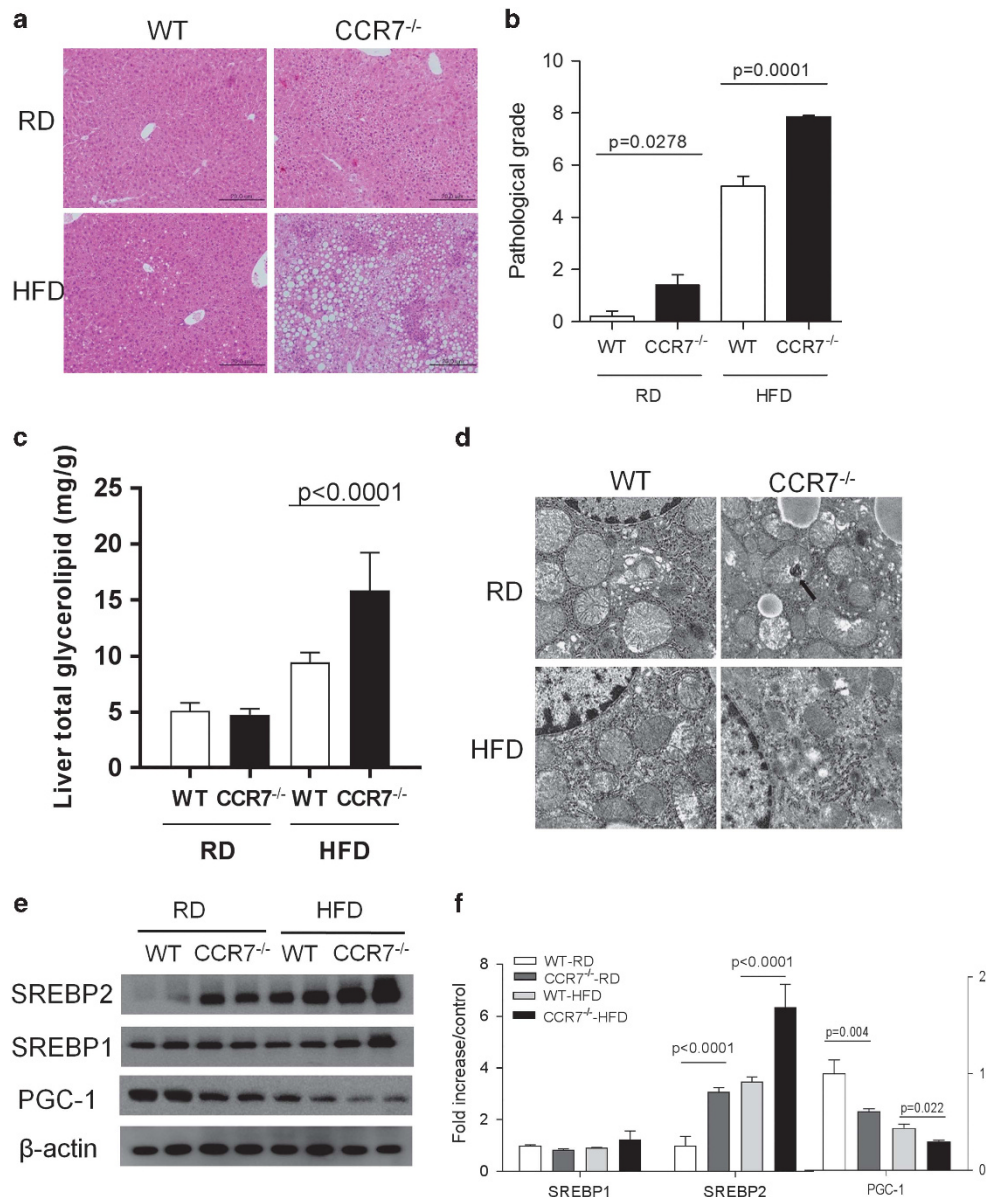
Figure 3. Glycerolipids content and liver steatosis were enhanced in high-fat diet CCR7 -/- mice. (a, b) Pathological grade from histological examination of the livers stained with hematoxylin and eosin. (c) Glycerolipids contents of the livers from RD- or HFD-fed WT and CCR7 -/- mice ( n = 10 /each group). (d) Electron microscopy analysis of mitochondria of hepatocytes from WT and CCR7 -/- mice (arrow = mitochondria damage). (e, f) Western blots of SREBP1, SREBP2 and PGC-1 in the liver. Cropped membrane was used in western blot. The band intensities were measured by Image J. Results shown are means \pm s.e.m. Abbreviation: SREBP, sterol regulatory element-binding protein.
