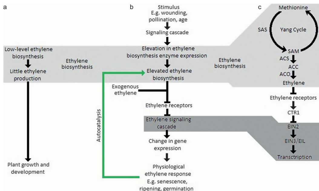
Figure 1. Simplified ethylene pathway. (a) Basal production of ethylene in the flowers during development before senescence. (b) The ethylene pathway upon triggering. The stimulus is translated to elevated ethylene synthesis producing higher levels of ethylene which inactivates the receptors initiating the signaling cascade which changes gene expression and finally induces physiological processes in the flower which may include the initiation of an autocatalytic loop. 14 (c) Simplified molecular events of the ethylene pathway. Methionine is enzymatically converted to S-adenosyl-L-methionine (SAM) by SAM synthase (SAS). SAM is partially converted back to methionine via several steps, but it also produces 1-aminocyclopropane-1-carboxylic acid (ACC) by ACC synthase (ACS). ACC is transformed to ethylene by ACC oxidase (ACO). Ethylene binds to receptors and stops their signal to CONSTITUTIVE TRIPLE RESPONSE1 (CTR1), which then stops its suppressing signal to ETHYLENE INSENSITIVE2 (EIN2). The released EIN2 is then cleaved and part of it is transported into the nucleus where activation of the ETHYLENE INSENSITIVE3/ETHYLENE INSENSITIVE3-LIKE (EIN3/EIL) transcription factor family occurs. This initiates a transcription cascade by activation of ETHYLENE RESPONSE FACTORS (ERFs) which eventually leads to differential gene expression and a physiological response. 15
