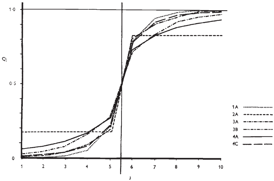
(a) s_1 = s_2 = 0.75 ; t_1 = t_2 = 1
