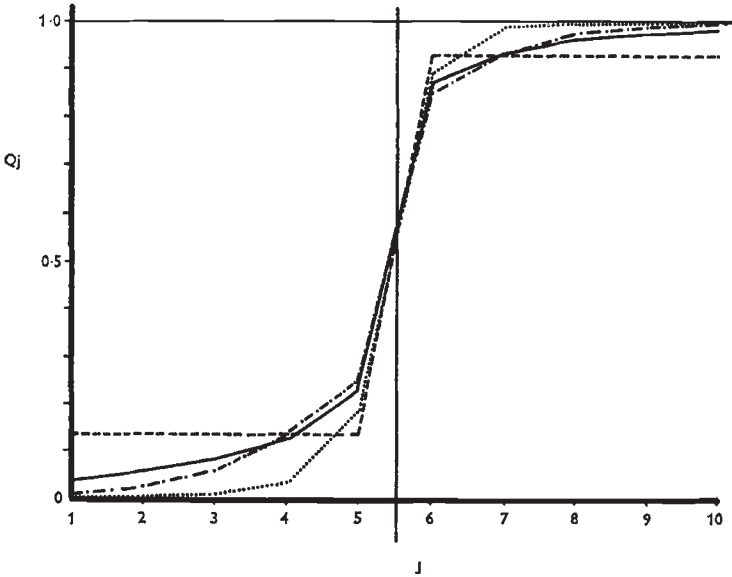
(b) s_1 = 0.95, s_2 = 0.50; t_1 = 1, t_2 = 5
