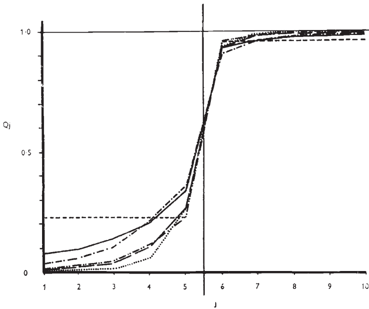
(b) s_1 = s_2 = 0.75 ; t_1 = 1 , t_2 = 5
