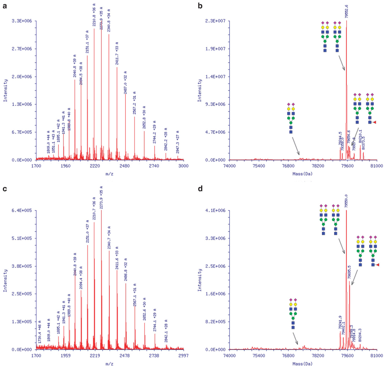
Figure 4 Mass spectra of affinity-purified Trf before (a, c, e, g) and after deconvolution (b, d, f, h). The structures of the oligosaccharides represented by the masses are indicated (blue squares = GlcNAc; green circles = Man; yellow circles = galactose; purple diamonds = sialic acid; red triangles = fucose). Panels a/b; representative mass data of Trf from the spleen obtained from an adult individual. Panels c/d; representative data from spleen samples from control fetuses. Panel e/f and g/h; representative data from spleen samples from affected fetuses, showing an abnormal peak of underglycosylated Trf.
