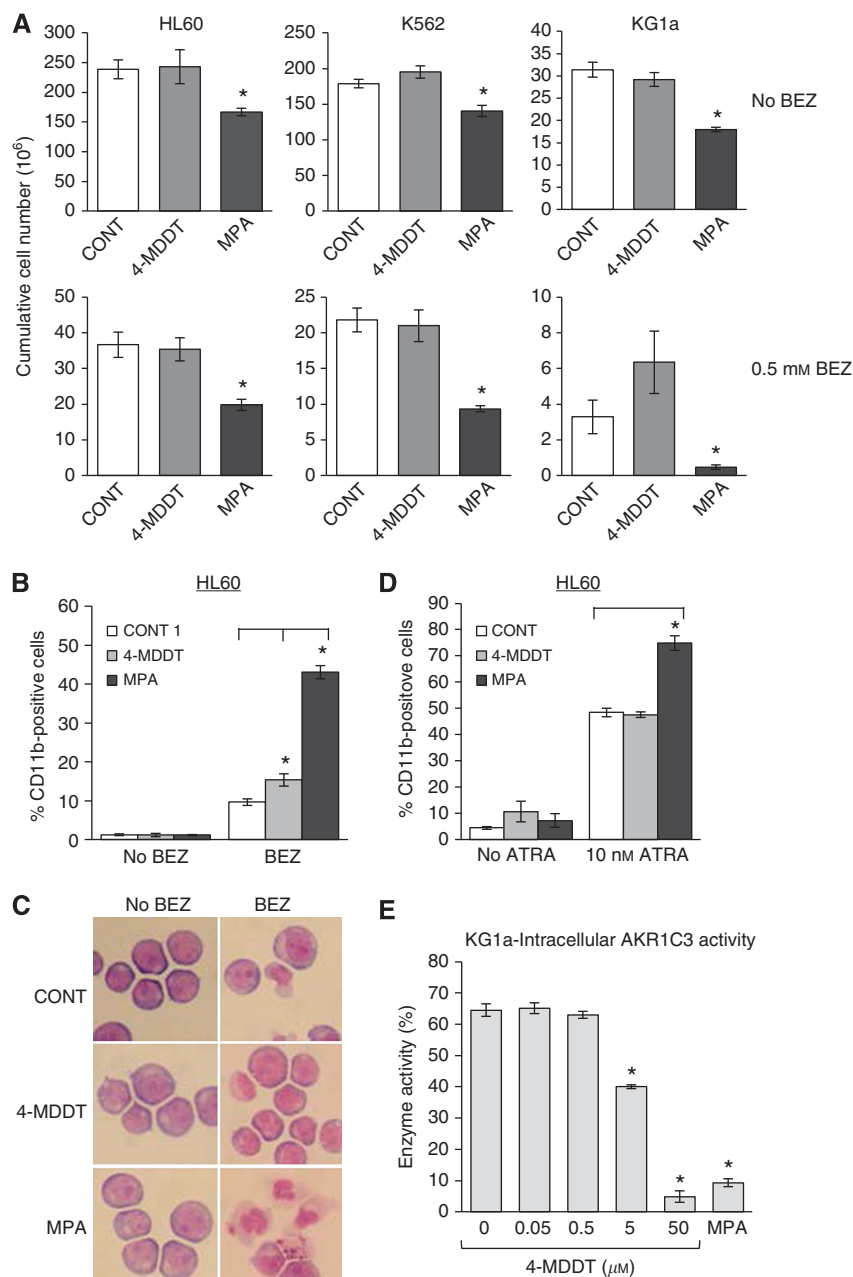
Figure 3. 4-MDDT does not recapitulate the actions of MPA against AML cell lines. HL-60, K562 and KG1a cells were treated for 7 days with either solvent control, 50 \mu\text{M} 4-MDDT or 5 \mu\text{M} MPA, alone or in combination with 0.5 mM BEZ. (A) Cumulative cell counts for HL60, K562 and KG1a after 7 days treatment. Data shown is mean of a minimum of N=3 experiments \pm s.e.m. (B and D) HL60 differentiation was assessed at day 7 by staining for CD11b and flow cytometry following treatment with either solvent control, 50 \mu\text{M} 4-MDDT or 5 \mu\text{M} MPA with or without 0.5 mM BEZ or 10 nM ATRA. Data shown is mean of a minimum of N=3 experiments \pm s.e.m. (C) Cytopsin of HL60 cells treated for 7 days as described above were stained with Jenner–Giemsa to demonstrate changes in cell morphology. (E) Intracellular AKR1C3 11 \beta -prostaglandin reductase activity in KG1a cells was assessed in the presence of a dose titration of 4-MDDT or 5 \mu\text{M} MPA using ^3\text{H} -PGD 2 and thin layer chromatography. Data shown is mean of N=4 experiments \pm s.e.m. * P<0.01 .
