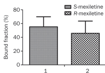
Figure 7. The binding of S-mexiletine (1) and R-mexiletine (2) (1.15 \mu\text{mol/mL} ) to HSA DOM II (4.9 \mu\text{mol/mL} ) ( n=3 ).
