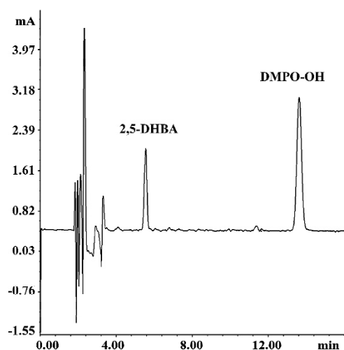
Figure 4. HPLC chromatograph of DMPO-OH adduct in \text{Fe}^{2+} -EDTA- \text{H}_2\text{O}_2 system.
