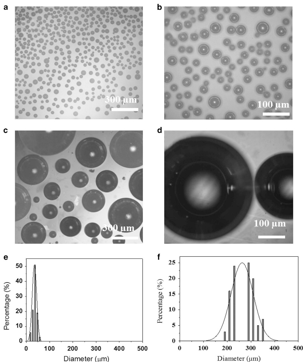
Figure 4 Digital images showing the size of N_2 bubbles produced on the electrode surface during hydrazine oxidation for (a, b) VGNH-45 and (c, d) FG. The corresponding statistical distributions of the bubble size are presented at the right for (e) VGNH-45 and (f) FG. These data clearly show that the bubble size released from VGNH-45 is approximately eight times smaller in diameter compared to those produced from the flat graphene electrode surface, which ultimately gives it 'superaerophobic' properties and hence results in its higher performance toward hydrazine oxidation.
