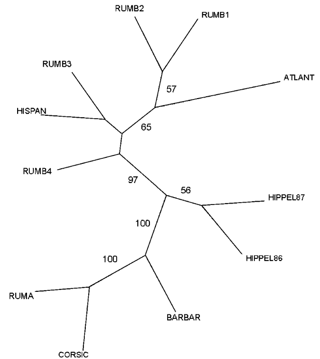
Figure 2 Unrooted maximum parsimony tree (unscaled) based on red deer mtDNA control region sequences observed on Rum ('RUM A' and 'RUM B1' – 'RUM B4') and across Europe and North Africa (see Table 1 for descriptions of sequence labels). Analyses excluded sites featuring indels. Percentage consensus from 1000 bootstrap replications of the data are shown for branches where these values were greater than 50%.
