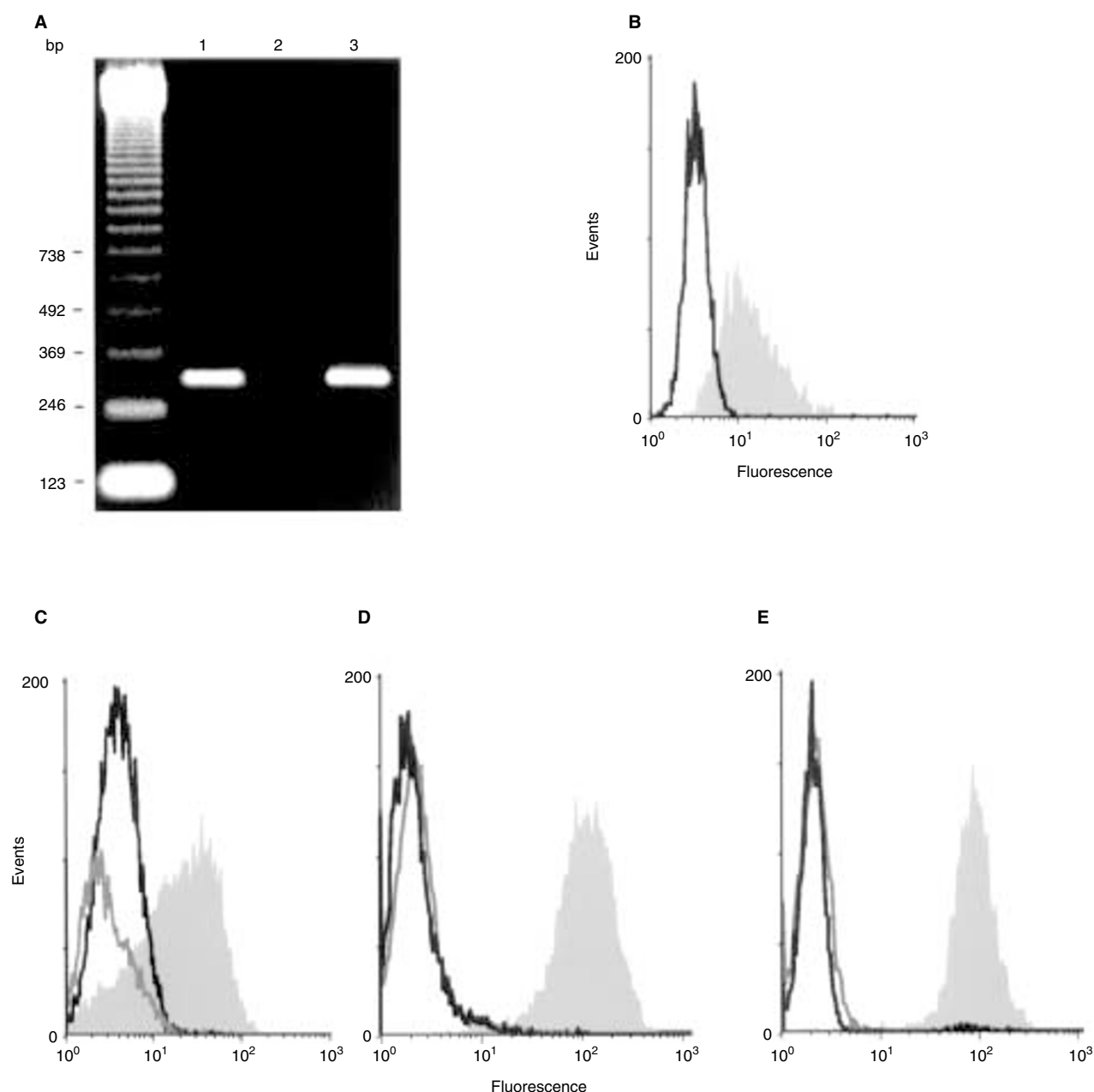
Figure 1 PBR mRNA and protein expression. (A) PBR mRNA expression in HT29 cells (lane 1) and in primary cell cultures of human colorectal cancers (lane 3) was detected by RT-PCR. Negative control was performed by omitting reverse transcriptase (lane 2). (B–E) Flow cytometric analysis of PBR expression in a primary cell culture of a colorectal cancer (B), and in the colorectal cell lines HT29 (C), LS174T (D), and Colo320 DM (E). Cells were stained with the specific PBR antibody 8D7 with previous membrane permeabilization (grey area) or without previous membrane permeabilization (grey line, C–E). Black line: isotypic control
