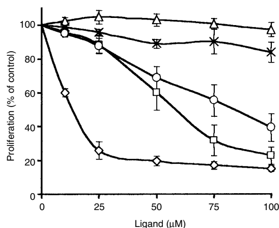
Figure 3 Antiproliferative effects of PBR ligands in HT29 cells. The specific PBR ligands FGIN-1-27 ( \diamond ), PK 11195 ( \square ), and Ro5-4864 ( \circ ) dose-dependently inhibited proliferation of HT29 cells as shown for a 72 h incubation period. Growth inhibition versus control was significant for FGIN-1-27 and Ro5-4864 from 10 \mu M to 100 \mu M, and for PK 11195 from 25 \mu M to 100 \mu M ( P < 0.05 ). In contrast, the GABA A -receptor ligand clonazepam ( \Delta ) or the 'no-affinity' ligand FGIN-1-52 ( \times ) showed no or only minor effects. Means of 4 to 6 independent experiments \pm SEM are shown
