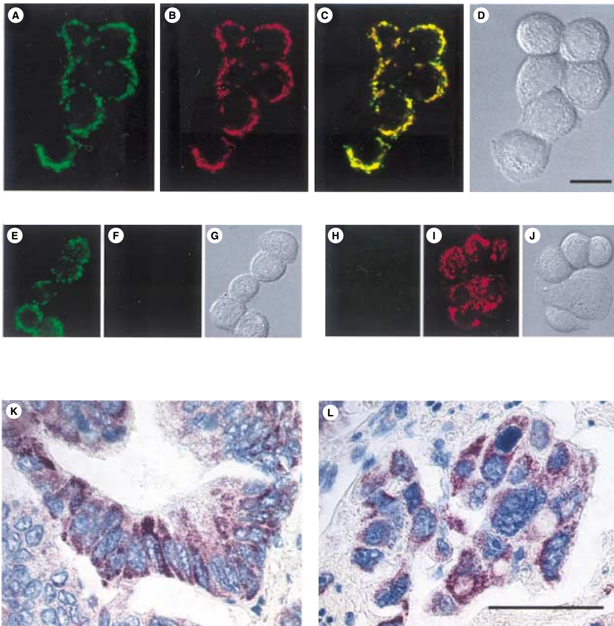
Figure 2 PBR localization in the mitochondria of HT29 cells. (A–J) Confocal laser scanning microscopy simultaneously visualized PBR and mitochondria. PBR was immunoassayed with the specific monoclonal antibody 8D7 (A, E), and mitochondria were marked with CMTMRos (B, I). Superposition of both fluorescence images resulted in a bright yellow colour (C), indicating a co-localization of PBR and mitochondria. Specificity of imaging was shown by omitting CMTMRos staining (F) or using isotypic control antibody (H), respectively. Corresponding transmission light images are shown (D, G, J). Bar = 10 \mu M. (K, L) Sections of paraffin-embedded tumours were immunohistochemically stained with anti-PBR antibody 8D7 and PBR expression was detected using the APAAP system (red colour). (K) Colorectal carcinoma classified as moderately differentiated. (L) Colorectal carcinoma classified as poorly differentiated. Bar = 100 \mu m
