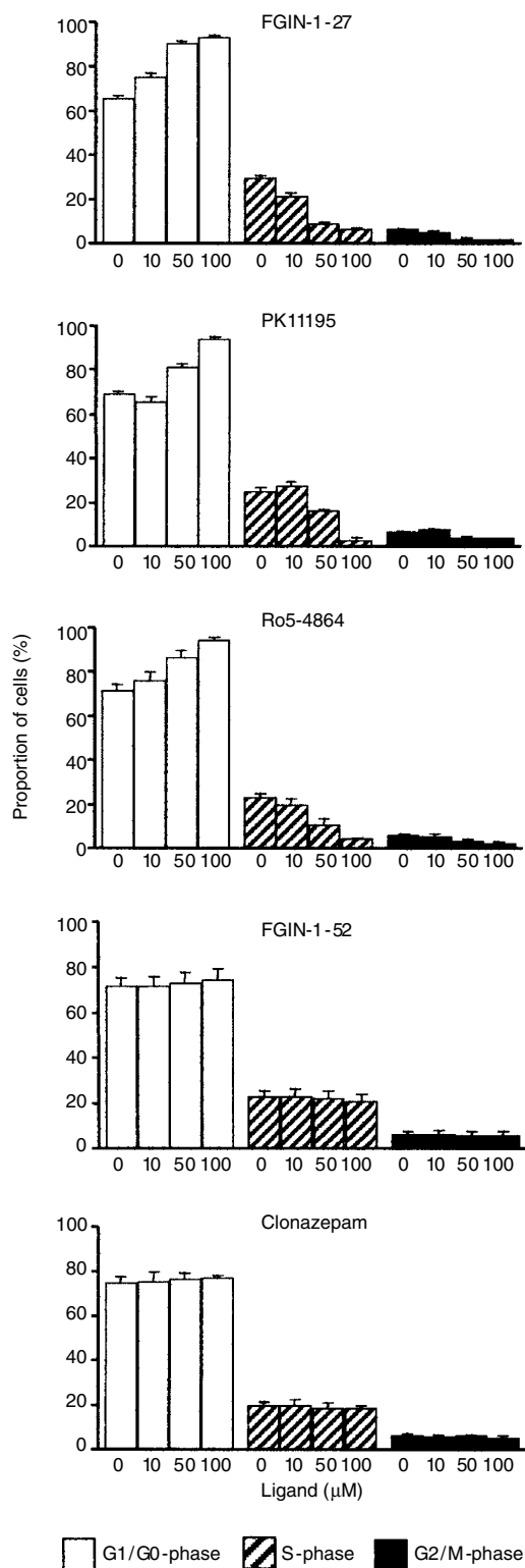
Figure 5 Induction of cell cycle arrest by PBR ligands. After 24 h of incubation the PBR ligands FGIN-1-27, PK 11195, or Ro5-4864, dose-dependently induced an arrest in the G 1 /G 0 -phase of the cell cycle (white columns), whereas the proportion of HT29 cells in S-phase (hatched columns) and G 2 /M-phase (black columns) decreased. FGIN-1-52, or clonazepam did not affect the cell cycle. Means \pm SEM of 3 independent experiments are shown. Difference of the proportion of cells in a respective phase of cell cycle versus control was significant for FGIN-1-27, PK 11195 and Ro5-4864 from 50 \mu M to 100 \mu M ( P < 0.05 )
