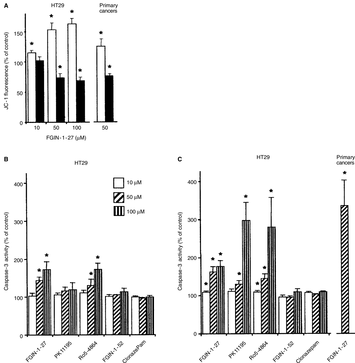
Figure 4 Induction of mitochondrial alterations and apoptosis by PBR ligands. (A) After 6 h of incubation with FGIN-1-27 \Delta\Psi_m (black columns) and mitochondrial volume (white columns) of HT29 cells and primary cultures of colorectal tumours were measured using the mitochondrial dye JC-1. \Delta\Psi_m is indicated by mean 590 nm: 530 nm fluorescence ratio, mitochondrial volume by mean 530 nm fluorescence. Means \pm SEM of 6 independent experiments with HT29 cells and of primary tumours from 6 patients are shown as percentage of control. * P < 0.05 versus control without agent. (B, C) HT29 cells were incubated for 6 h (B) or 16 h (C) with 10 \mu M to 100 \mu M of FGIN-1-27, PK 11195, Ro5-4864, FGIN-1-52, or clonazepam and caspase-3 activity was determined. Means as percentage of control \pm SEM of 4 independent experiments are shown. In addition, caspase-3 activity was determined of primary tumour cells of 6 patients after incubation with 50 \mu M FGIN-1-27. Mean \pm SEM are shown. * P < 0.05 versus control without agent
