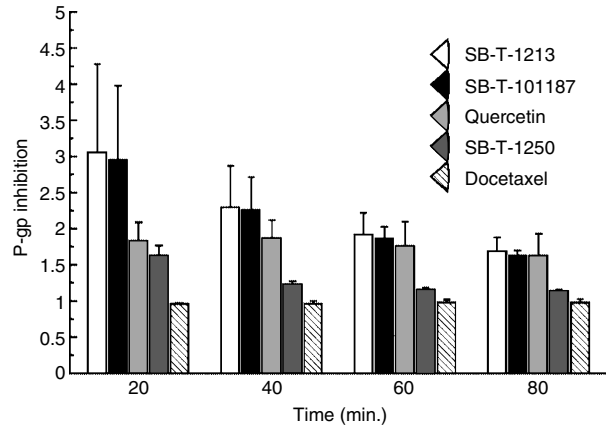
Figure 5 Bar chart of P-gp inhibition of the panel of taxanes. MCF-7 ADRr cells were loaded with Rh123 (0.5 \mu M). After 15 min., cells were transferred onto ice and washed twice in cold PBS/BSA 0.2%. On to ice was added 10 \mu M of all the tested drugs or the vehicle DMSO 0.1%. Cells were then kept at 37°C to allow the maximal dye efflux. An aliquot of cells was maintained on ice to have the maximal dye uptake. At each time point (from 20 to 80 min), Rh123 fluorescence was assessed by flow cytometry. The ratio between control at 37°C and control at 4°C served to calculate the control dye efflux. The same procedure was employed for each drug. This ratio was divided by the amount of the control dye efflux. A value higher than 1 means that drug acts as P-gp inhibitor. Results obtained from the mean of two independent experiments are shown. Bars represent the standard deviations
