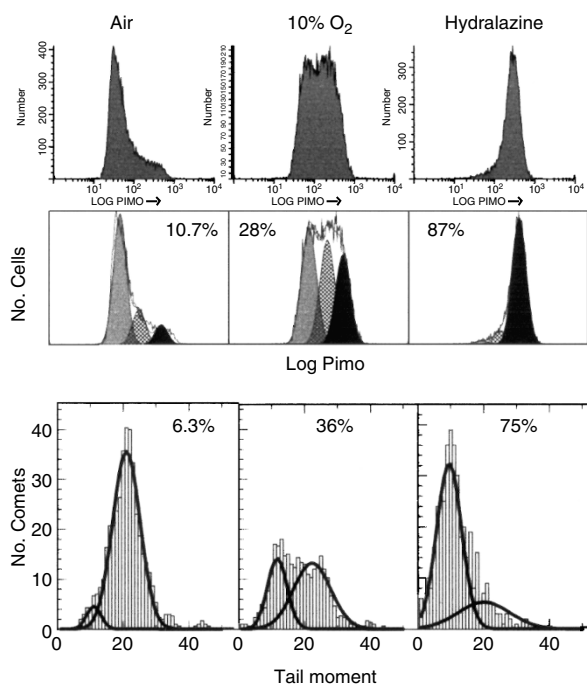
Figure 2 Representative data from 3 SCCVII tumours analysed for pimonidazole binding and DNA damage. The upper curves show the distributions of anti-pimonidazole antibody binding in tumours from a mouse breathing air, 10% oxygen in nitrogen, or treated with hydralazine to reduce tumour blood flow. A fitting program was used to describe 3 normally distributed populations representing aerobic, intermediate and hypoxic tumour cells. The percentage of hypoxic cells is shown in the middle panels. For the same tumours, cells were analysed for hypoxic fraction using the comet assay that detects the difference in radiation-induced strand breaks between aerobic and radiobiologically hypoxic tumour cells. The percentage of hypoxic cells is given in each panel
