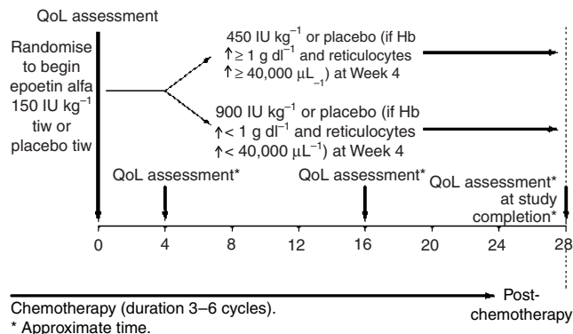
Figure 1 Study schema.
