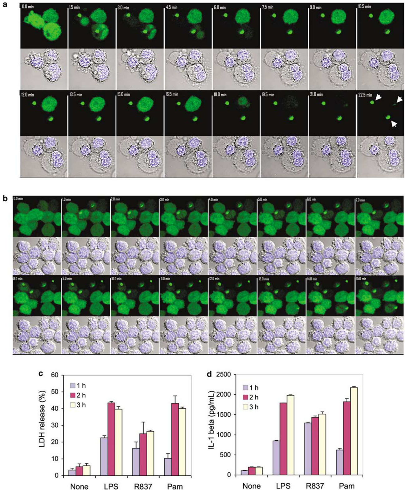
Figure 2 Formation of the ASC pyroptosome causes cell death in THP-1 cells. ( a and b ) Time-series confocal images ( \times 63 magnification) of crude LPS-stimulated THP-1-ASC-GFP cells in the absence ( a , 1.5 min images are shown) or presence of zVAD-FMK ( 70 \mu\text{M} ) ( b , 1.0 min images are shown). The arrows in the last image point to ASC pyroptosomes. Time-lapse movies showing the assembly of the ASC pyroptosome in the absence or presence of zVAD-FMK can be seen in the 'Supplementary Movies 1–5'. ( c and d ) Pyroptosome-induced pyroptosis causes the release of intracellular LDH and IL- 1\beta . PMA-primed parental THP-1 or THP-1-ASC-GFP cells were pretreated for 1 h with ultrapure LPS to induce pro-IL- 1\beta and then treated with crude LPS ( 1.0 \mu\text{g/ml} ), R837 ( 10 \mu\text{g/ml} ) or Pam3CSK4 ( 0.5 \mu\text{g/ml} ) for the indicated periods of time. LDH release into the culture medium is shown as a percentage of LDH release by detergent ( c ). IL- 1\beta release into the culture media was determined by ELISA ( d )
