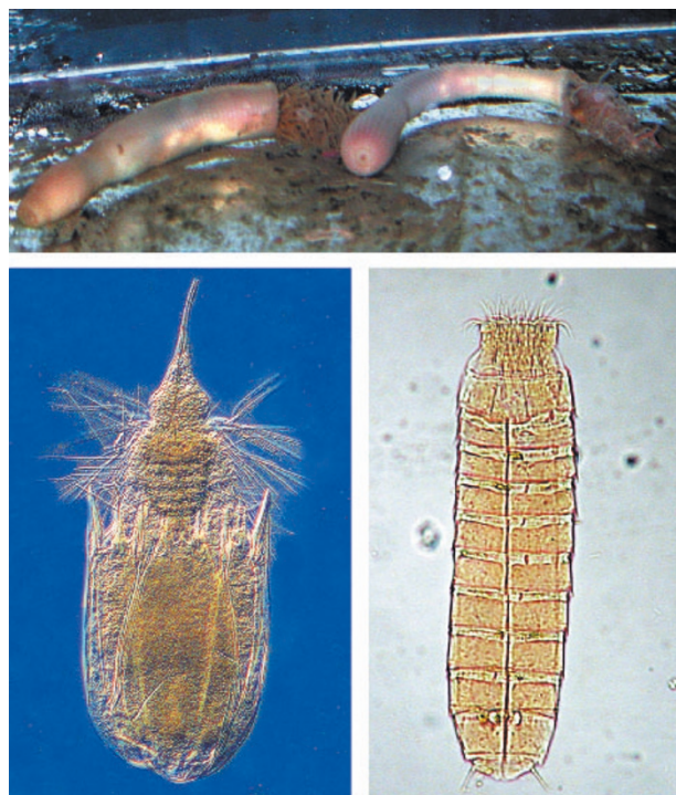
Figure 1 Adult representatives of the three living scalidophorans. Top, two specimens of the priapulid Priapulus caudatus (length about 10 cm). Bottom left, the loriferan Nanaloricus mysticus (0.3 mm). Bottom right, the kinorhynch Pycnophyes kielensis (0.7 mm). The Cambrian embryo Markuelia , the subject of Dong and colleagues' analysis 5 , seems to be more primitive than any of these very diverse worms. (Images of Nanaloricus by R. M. Kristensen, and of Priapulus and Pycnophyes by G. E. Budd.)
