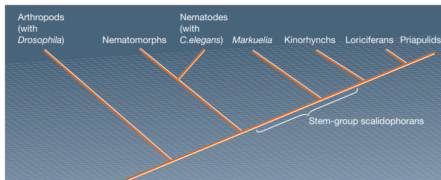
Figure 2 The place of Markuelia in evolution, as inferred from the new work 5 . The positions of the two major model organisms, C. elegans and Drosophila , are also indicated. Nematomorphs are a group of parasitic worms closely related to the nematodes.
