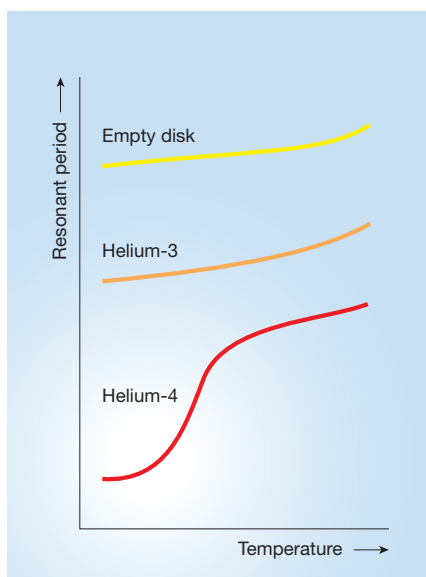
Figure 1 Super solid. Kim and Chan 8 suspended a porous Vycor glass disk (15 mm in diameter and 4 mm thick) containing solid helium-4 in a torsional oscillator and monitored the disk's rotational inertia as the temperature decreased. Below about 175 mK they saw a sharp drop in the resonant period of oscillations, which is related to the disk's inertia. No such effect was seen for a Vycor disk empty of helium-4, or when the disk was filled with helium-3. Helium-4 was the first superfluid to be discovered; this might be the first evidence of supersolid behaviour.
