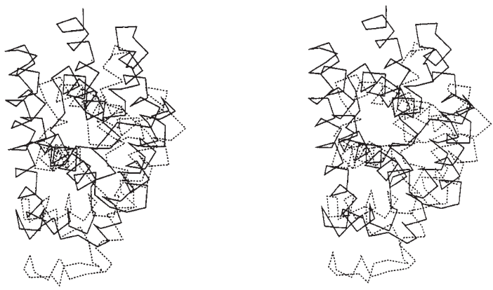
FIG. 2 Stereo view of superimposed C\alpha traces of colicin A and myoglobin (shown dashed). The amino terminus of myoglobin is at the upper right, that of colicin A at the lower left.
