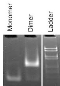
Figure 3(e) The high-efficiency formation of pRNA dimer was demonstrated by native-PAGE.
