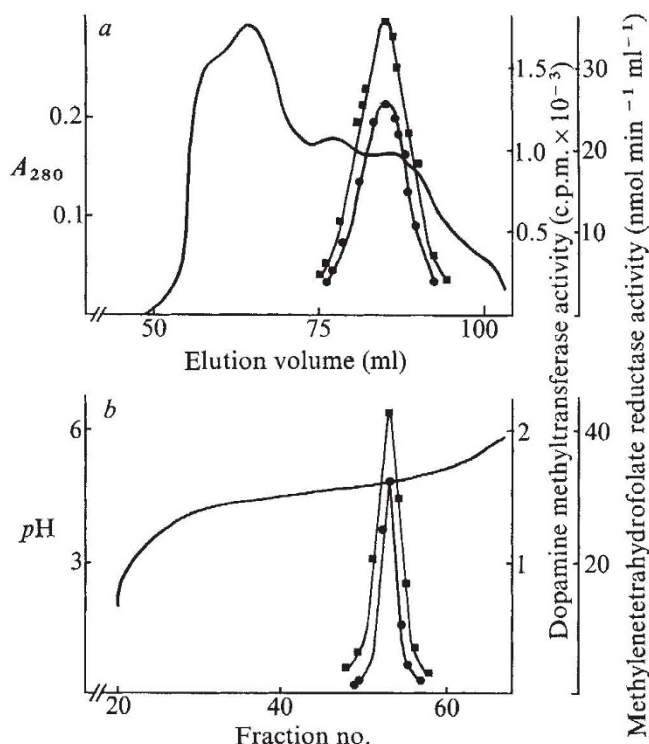
Fig. 2 a , Isolation of methylenetetrahydrofolate reductase by gel filtration on Sephadex G-200. 10 mg methylenetetrahydrofolate reductase (specific activity, 0.1 U mg -1 ) purified from pig liver by the method of Kutzbach and Stokstad 11 was applied to a Sephadex G-200 column (1.5 × 95 cm) equilibrated in 10 mM potassium phosphate buffer, pH 7.5 containing 1 mM EDTA and 1 mM mercaptoethanol. Fractions were assayed for protein (A 280 ) and for methylenetetrahydrofolate reductase (●) and dopamine methyltransferase (■) activities as described in the text. b , Isoelectric focusing of methylenetetrahydrofolate reductase. 10 mg methylenetetrahydrofolate reductase was electrofocused at 4 °C in a 110 ml LKB column using ampholine, pH 3.5–5.0, in a 20–60% glycerol gradient. When electrofocusing was complete the column was drained and 2 ml fractions were collected. The pH value and the activities of methylenetetrahydrofolate reductase (●) and dopamine methyltransferase (■) of the fractions were measured. The recovery of enzyme activity was 50–60%.
