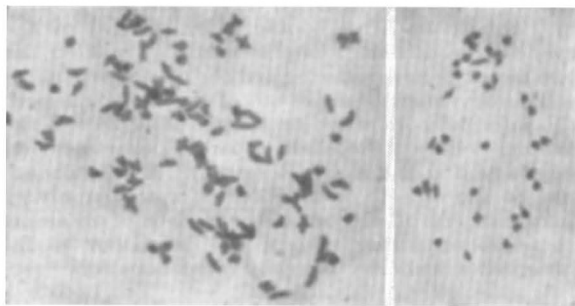
MEIOTIC METAPHASES IN ACETOCARMINES OF A HEXAPLOID AND A DIPLOID Polypodium . \times 500 . (a) MORPHOLOGICALLY NORMAL SPECIMEN FROM WINDERMERE; (b) THE HORTICULTURAL VARIETY 'SEMILACERUM'
