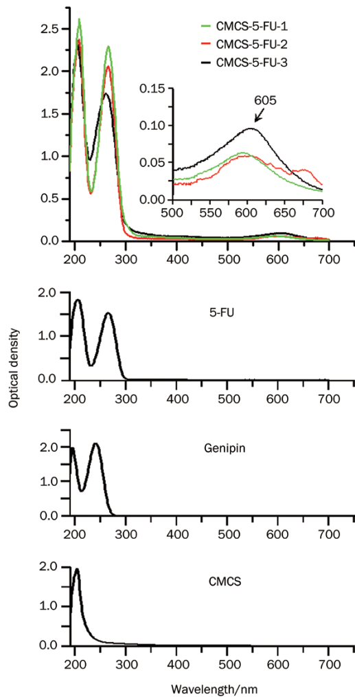
Figure 3. UV-vis spectra of the 5FU-loaded CMCS hydrogels, 5FU, genipin, and CMCS.
