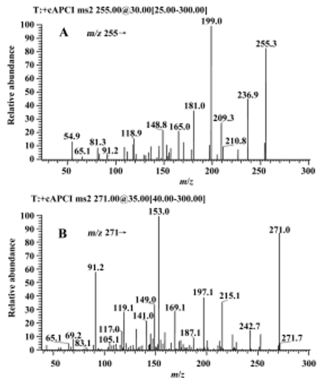
Figure 2. Full-scan product-ion spectra of [M + H]^+ of (A) daidzein and (B) genistein.
